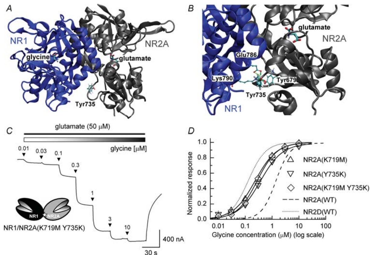
Figure 9. Analysis of the effects of point mutations in the S2 region of the NR2A subunit on glycine potency
