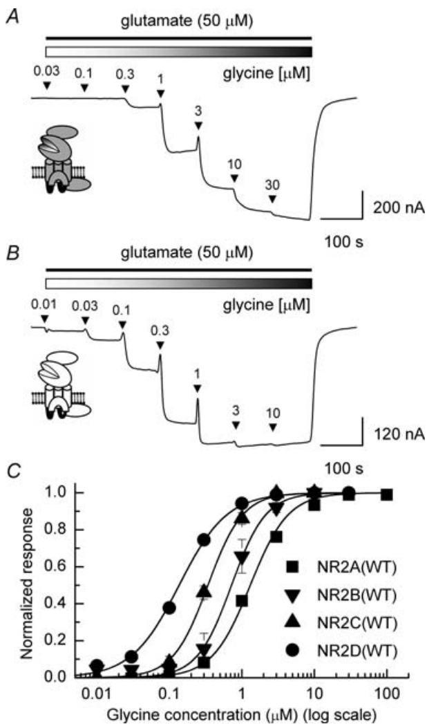
Figure 2. Example TEVC current traces showing responses evoked by increasing concentrations of glycine for NR1/NR2A and NR1/NR2D NMDARs
