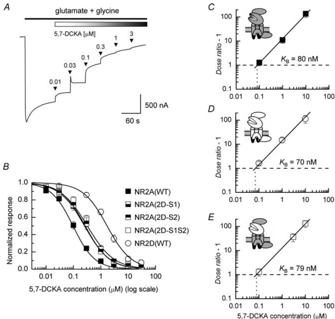
Figure 7. Antagonism of wild-type and chimeric NMDAR mediated responses by 5,7-DCKA
