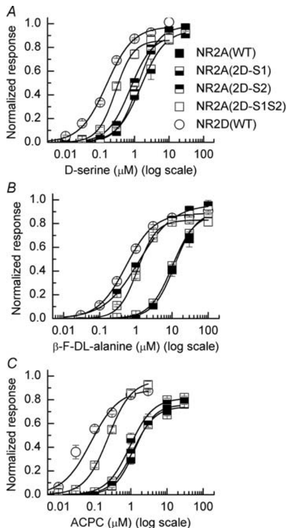
Figure 5. Concentration–response curves for D-serine, \beta -fluoro-DL-alanine and ACPC acting at wild-type and chimeric NMDARs
