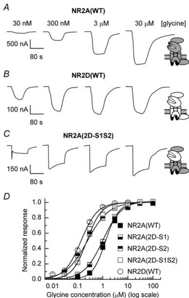
Figure 4. Glycine concentration–response data for wild-type and chimeric NMDARs
