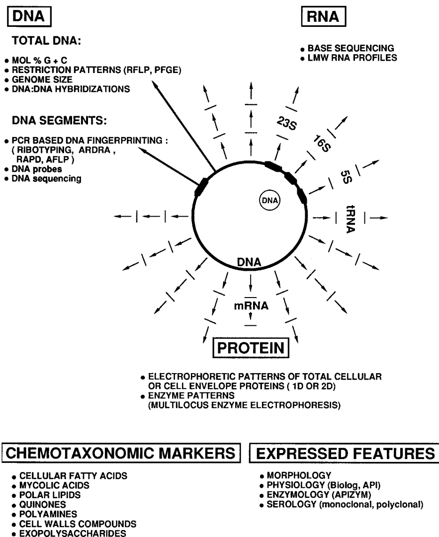
FIG. 1. Schematic overview of various cellular components and techniques used. RFLP, restriction fragment length polymorphism; PFGE, pulsed-field gel electrophoresis; ARDRA, amplified rDNA restriction analysis; RAPD, randomly amplified polymorphic DNA; AFLP, amplified fragment length polymorphism; LMW, low molecular weight; 1D, 2D, one- and two-dimensional, respectively.
