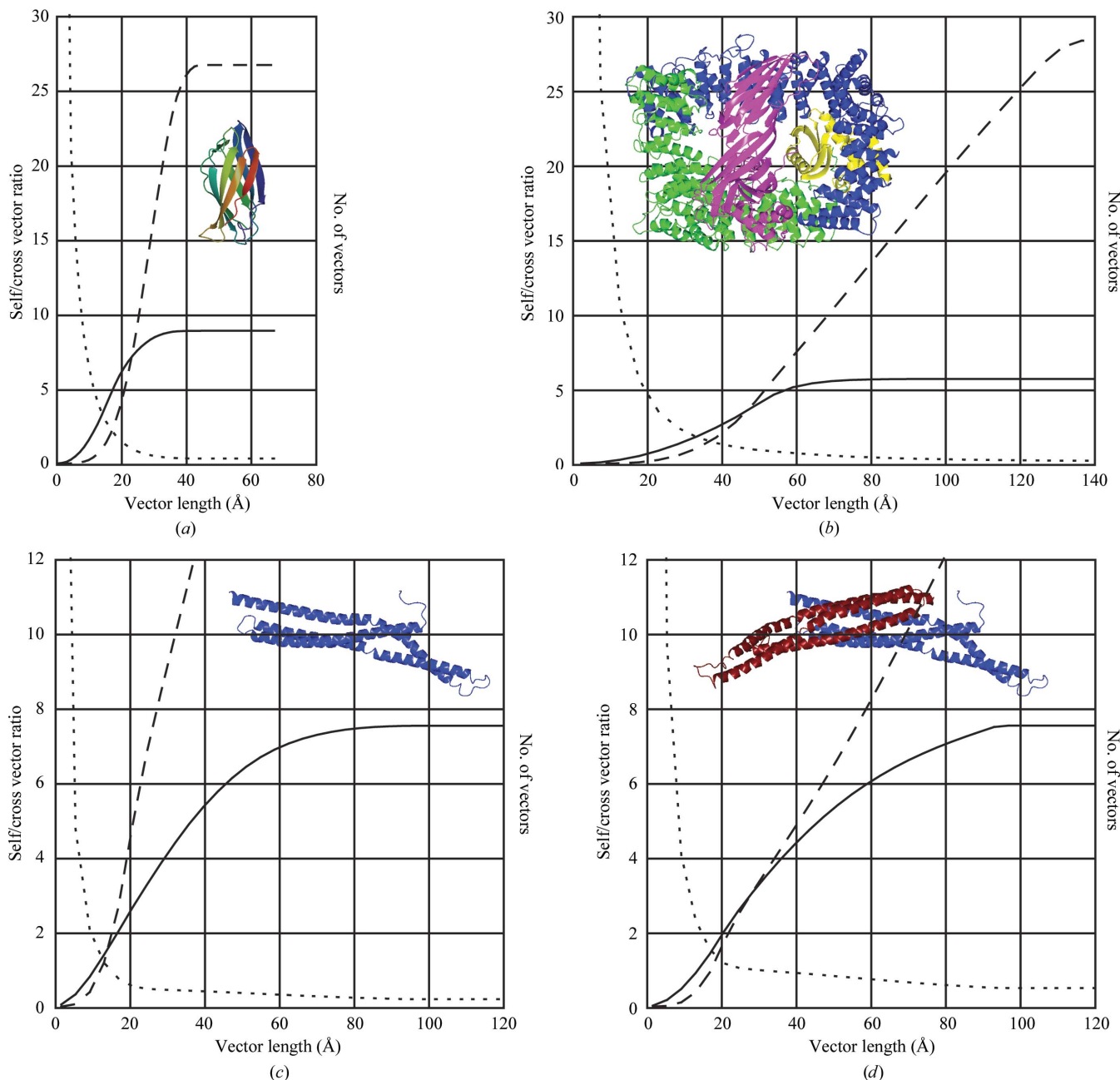
Figure 1 The separation between self-vectors and cross-vectors as a function of vector length (radius from the Patterson origin) for some example structures. In each case, the solid line is the number of self-vectors, the dashed line is the number of cross-vectors and the dotted line is the self/cross vector ratio. (a) A small protein, 119 residues, size \sim 23 \times 23 \times 50 Å, space group P2_12_12_1 , PDB code 1gyu. (b) A larger heterotetramer, 1730 residues, \sim 80 \times 80 \times 100 Å, space group P3_12_1 , PDB code 1gw5. (c) An elongated monomer, 217 residues, \sim 25 \times 25 \times 110 Å, space group P3_12_1 , PDB code 1uru. (d) The equivalent dimer, 434 residues, \sim 25 \times 25 \times 145 Å, calculated in space group P3_1 .
