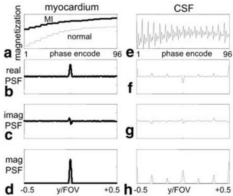
FIG. 2. Simulated magnetization recovery and corresponding PSFs for segmented acquisition with interleaved phase order. Normal and infarcted (bold) myocardia are shown in a–d , and CSF is shown in e–h . The transient approach to steady state for CSF with long T_1 causes ghost artifacts.
