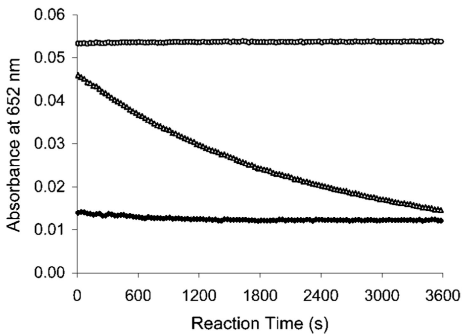
Figure 4. Plot of absorbance at 652 nm versus time of Lu(III)-AAIH ( \circ ), Lu(III)-C-DOTA ( \Delta ), Lu(III)-C-NETA ( \blacklozenge ) at pH 4.5 (0.15 M \text{NH}_4\text{OAc} ) and 25 ^\circ\text{C} .
