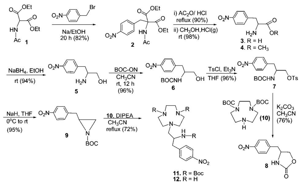
Scheme 2. Synthesis of Precursor Molecule 12 for C-NETA
