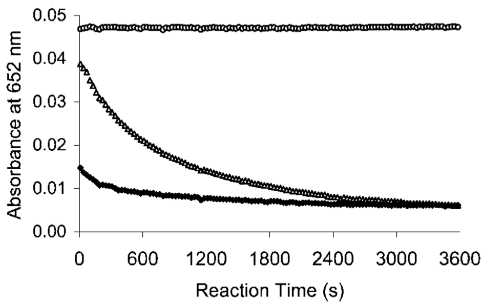
Figure 3. Plot of absorbance at 652 nm versus time of Bi(III)-AAIH (○), Bi(III)-C-DOTA (△), Bi(III)-C-NETA (◆) at pH 4.0 (0.15 M \text{NH}_4\text{OAc} ) and 25 °C.
