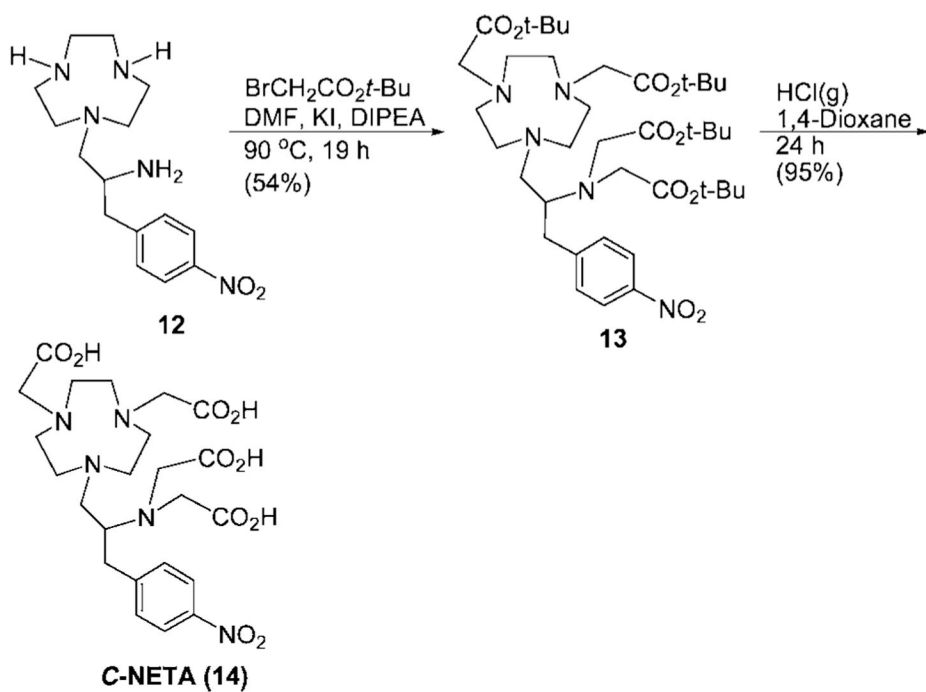
Scheme 3. Synthesis of C-NETA
