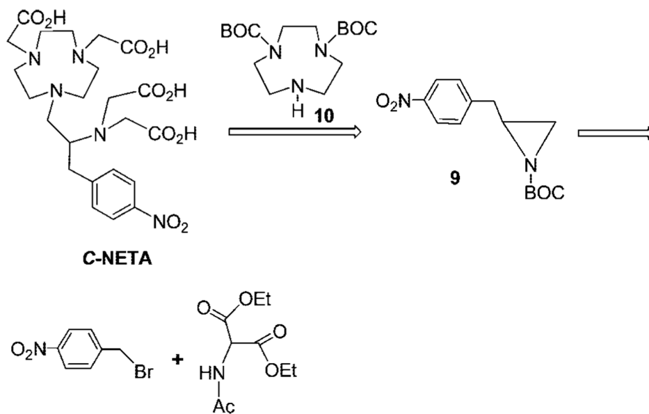
Scheme 1. Retrosynthetic Route to C-NETA
