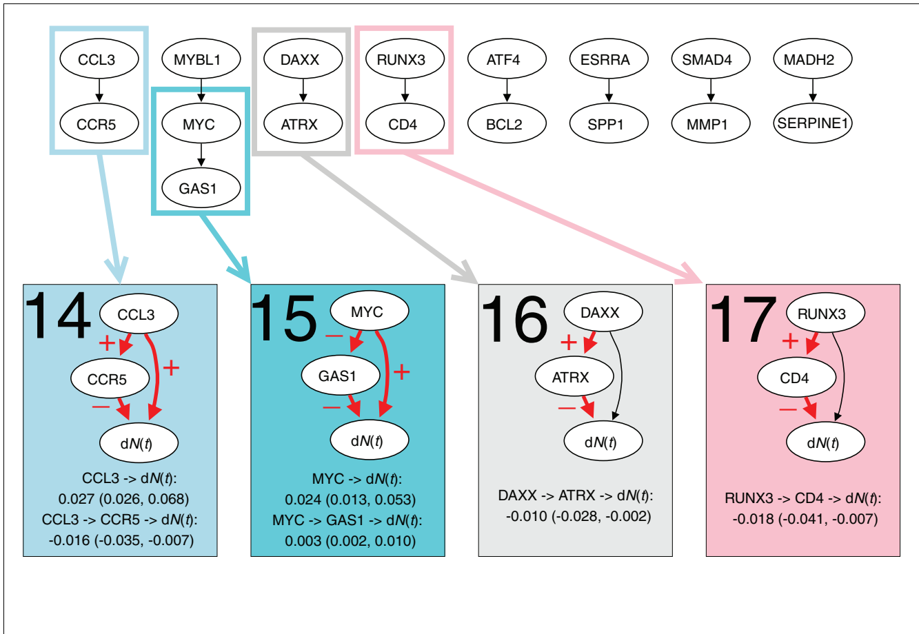
Figure 6 Dynamic path models for the DLBCL data set. The top panel shows the thinned survival forest after selecting genetic interactions for which an indirect and direct effect likely existed. Black arrows indicate a total of nine significant interactions. The thinned forest consisted of eight networks. A number of dynamic path models were fitted to different sub-networks of these networks: each connected component, each rooted subtree (that is, each gene with all of its descendants), and each interaction separately. For ten models there was at least one significant indirect effect, indicated with rectangles of different colors. Below the thinned forest, the ten models with at least one significant indirect effect are shown. Interactions with significant direct or indirect effects are marked with red arrows. The plus and minus signs on arrows between two genes indicate transcriptional activation and repression, respectively, whereas the plus and minus signs on arrows pointing to survival ( dN(t) ) indicate that poor survival is associated with activation and repression of the gene, respectively. For each significant path, the average strength of the direct and indirect effect during the first five years is listed, along with a 95% bootstrap confidence interval.
