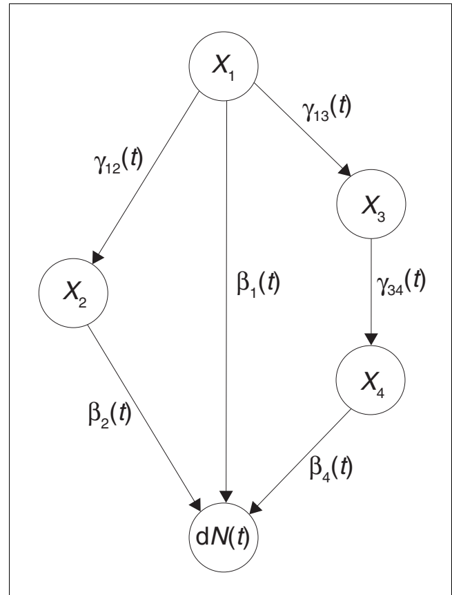
Figure 7 The dynamic path model with direct and indirect effects. This figure shows a dynamic path model with four covariates (genes) X_1, X_2, X_3 and X_4 illustrating how the strength of the direct and indirect effect of X_1 on survival dN(t) is calculated. Interactions between the covariates are shown as arrows (edges). Each \gamma_j(t) is an ordinary least squares regression coefficient at time t , and each \beta_j(t) is an additive hazard regression coefficient at time t . The strength of the direct effect of X_1 on dN(t) is given by \beta_1(t) . There are two indirect paths from X_1 to dN(t) : one through X_2 and one through X_3 and X_4 . The strength of the indirect effect of X_1 on dN(t) is therefore given by \gamma_{12}(t)\beta_2(t) + \gamma_{13}(t)\gamma_{34}(t)\beta_4(t) . The strength of the total effect is the sum of the strength of the direct and indirect effect, that is, \beta_1(t) + \gamma_{12}(t)\beta_2(t) + \gamma_{13}(t)\gamma_{34}(t)\beta_4(t) .
