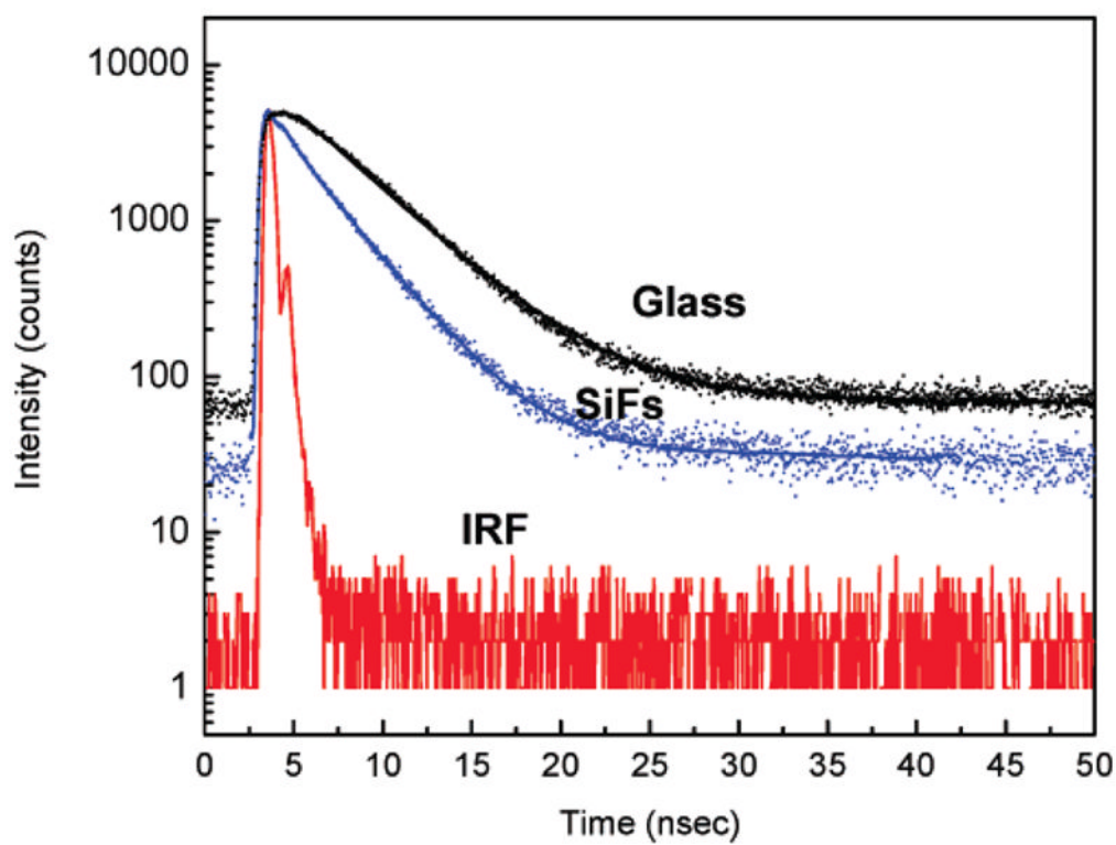
Figure 5. Fluorescence intensity decays from a liquid sandwich of R-phycoerythrin on glass and SiFs. IRF = instrument response function. SiFs = silver island films.
