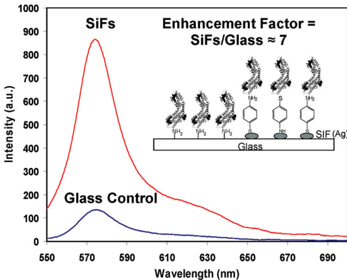
Figure 1. Fluorescence emission spectra from a monolayer of R-phycoerythrin on glass and SiFs. (Inset) Experimental configuration. SiFs = silver island films.
