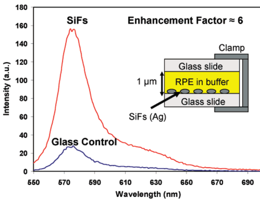
Figure 4. Fluorescence spectra from a liquid sandwich of R-phycoerythrin on glass and SiFs. (Inset) Diagram showing experimental configuration.
