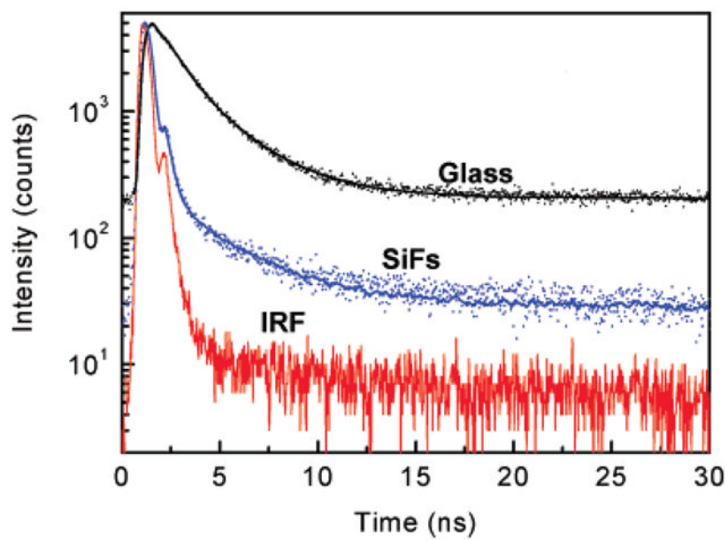
Figure 2. Fluorescence intensity decays from a monolayer of R-phycoerythrin on glass and SiFs. IRF = instrument response function. SiFs = silver island films.
