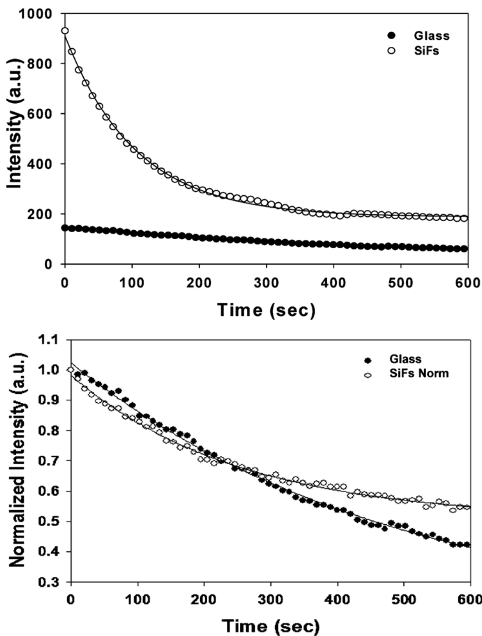
Figure 3. (Top) Steady-state fluorescence intensity decays from a monolayer of R-phycoerythrin on glass and SiFs. (Bottom) Normalized intensity decays for a monolayer of R-phycoerythrin on glass and SiFs after the incident laser power on SiFs was adjusted to match the initial fluorescence signal intensity on glass.
