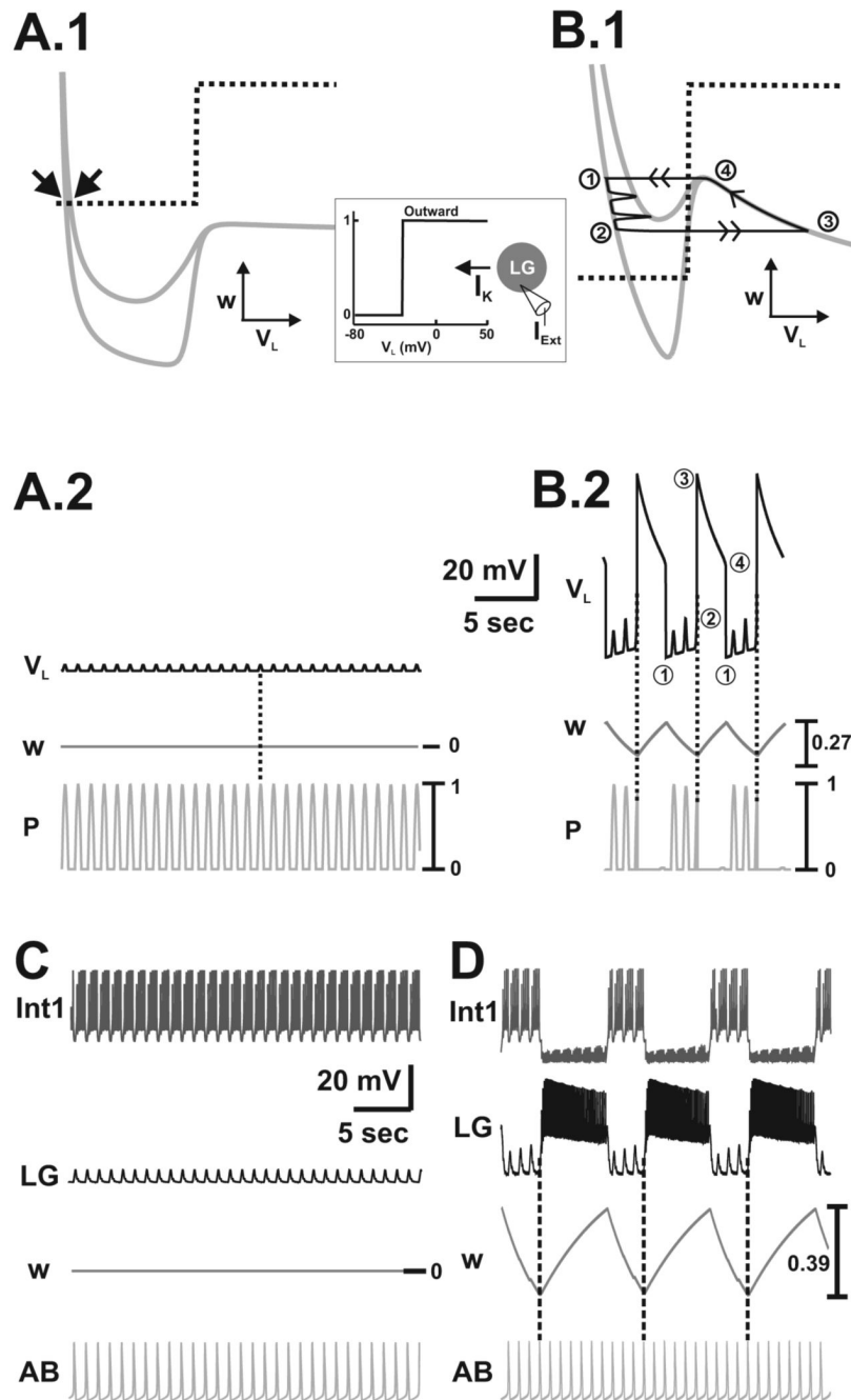
Figure 6. Network oscillations with only I_K in the LG neuron (as shown by schematic inset) induced by depolarizing DC current injection. A.1-A.2 , When I_{Proc} is removed from the model (by setting \bar{g}_{Proc} = 0 \text{ mS/cm}^2 in Equations (21): PK mechanism 2) the V_L - and w -nullclines intersect at stable fixed points (arrows in A.1 ) so that network oscillations can not occur. V_L exhibits small, pyloric-timed depolarizations (dotted line in A.2 ), but the LG neuron remains in its inactive state. Most hyperpolarized LG membrane potential: -77 \text{ mV} . B.1-B.2 , Injecting external current ( I_{Ext} = 150 \mu\text{A/cm}^2 ) into the LG neuron moves the intersection of the V_L - and w -nullclines to the middle branch of the cubic so that network oscillations occur ( B.1 ). As in Figure 5, the slow activation variable w of I_K controls the network oscillations and the onset
