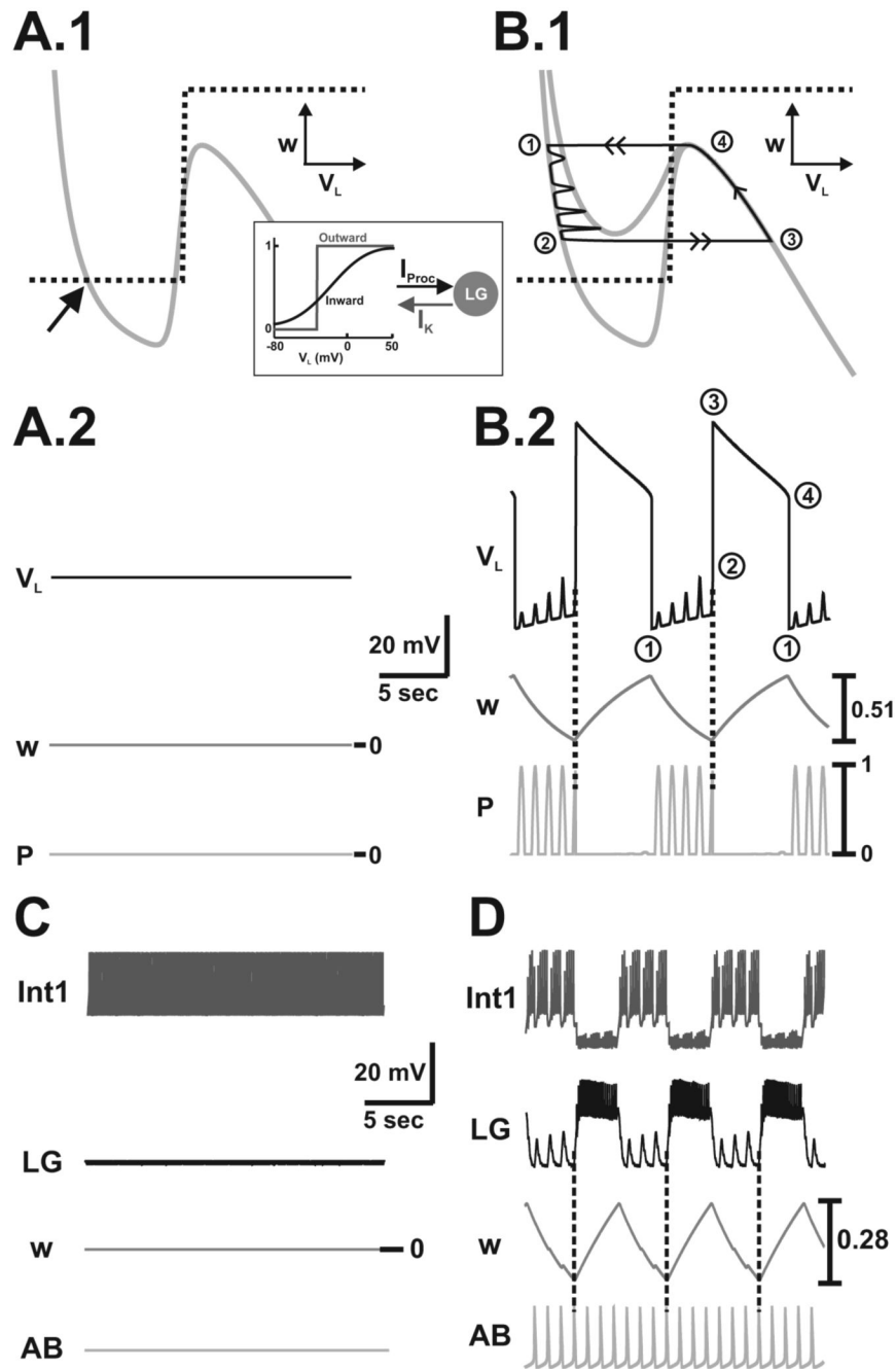
Figure 5. PK-elicited gastric mill rhythm (mechanism 2: PK induces I_{Proc} and I_K in the LG neuron as shown in the schematic inset). I_{Proc} is a fast inward current while I_K is a slow outward current. Both currents are non-inactivating. Network oscillations are driven by the slow activation variable ( w ) of I_K . A.1-A.2 , The cubic shape of the V_L -nullcline is inverted in the V_L - w phase plane ( A.1 ). In the absence of the pyloric input, the V_L - and w -nullclines intersect at a stable fixed point along the left branch of the cubic in the V_L - w phase plane (indicated by arrow in A.1 ). As a result, the LG neuron remains in its inactive state, and network oscillations can not be elicited without the pyloric input ( A.2 ; most hyperpolarized LG membrane potential: -55 mV). B.1-B.2 , In the presence of the pyloric input, PK-induction of I_{Proc} and I_K in the LG
