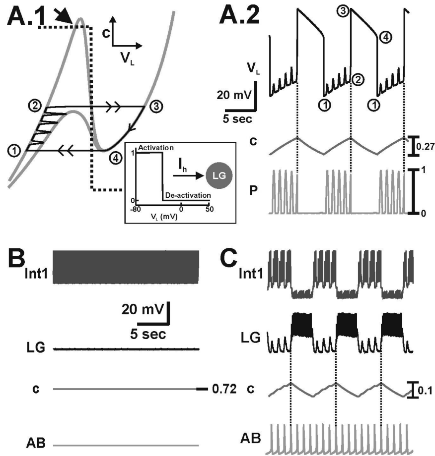
Figure 7. PK-elicited gastric mill rhythm (mechanism 3: PK induces I_h in the LG neuron). A.1-A.2 , Network oscillations do not occur in the unforced system since the V_L - and c -nullclines intersect along the stable left branch of the higher cubic (arrow in A.1 ). In the forced system, the induction of I_h in the LG neuron (as indicated in the schematic inset) elicits a gastric mill rhythm ( A.2 ) controlled by the activation variable c of I_h . In the V_L - c phase plane, the trajectory slowly climbs up the left branch of the V_L -nullcline as it is moved back and forth between the unforced and maximally forced cubics by the pyloric input ( A.1 ). As a result, c slowly increases during the inactive state of the LG neuron and slowly depolarizes V_L ( A.2 ). At point 2, the V_L -nullcline is shifted below the phase point by a pyloric peak, which initiates the jump to the right branch of the cubic ( A.1 ) and determines the onset of the LG active state (dotted lines in A.2 ). During the active state of the LG neuron, the trajectory slowly falls down the right branch of the V_L -nullcline ( A.1 ) and c slowly decreases in the LG neuron to repolarize V_L ( A.2 ). At point 4, the trajectory jumps back to the left branch ( B.1 ) and the cycle repeats. Most hyperpolarized LG membrane potential: -66 mV. B-C , In the biophysically-realistic model, hyperpolarizing the AB neuron inactivates the AB to Int1 synapse which does not allow for the generation of a gastric mill rhythm ( B ). In the presence of this synapse, the gastric mill rhythm is driven by the dynamics of I_h in the LG neuron ( C ). Vertical dotted lines in C indicate the onsets of LG bursts. Most hyperpolarized membrane potentials: Int1 -48 mV ( B ), -61 mV ( C ); LG -49 mV ( B ), -52 mV ( C ), AB -65 mV ( B ), -64 mV ( C ).
