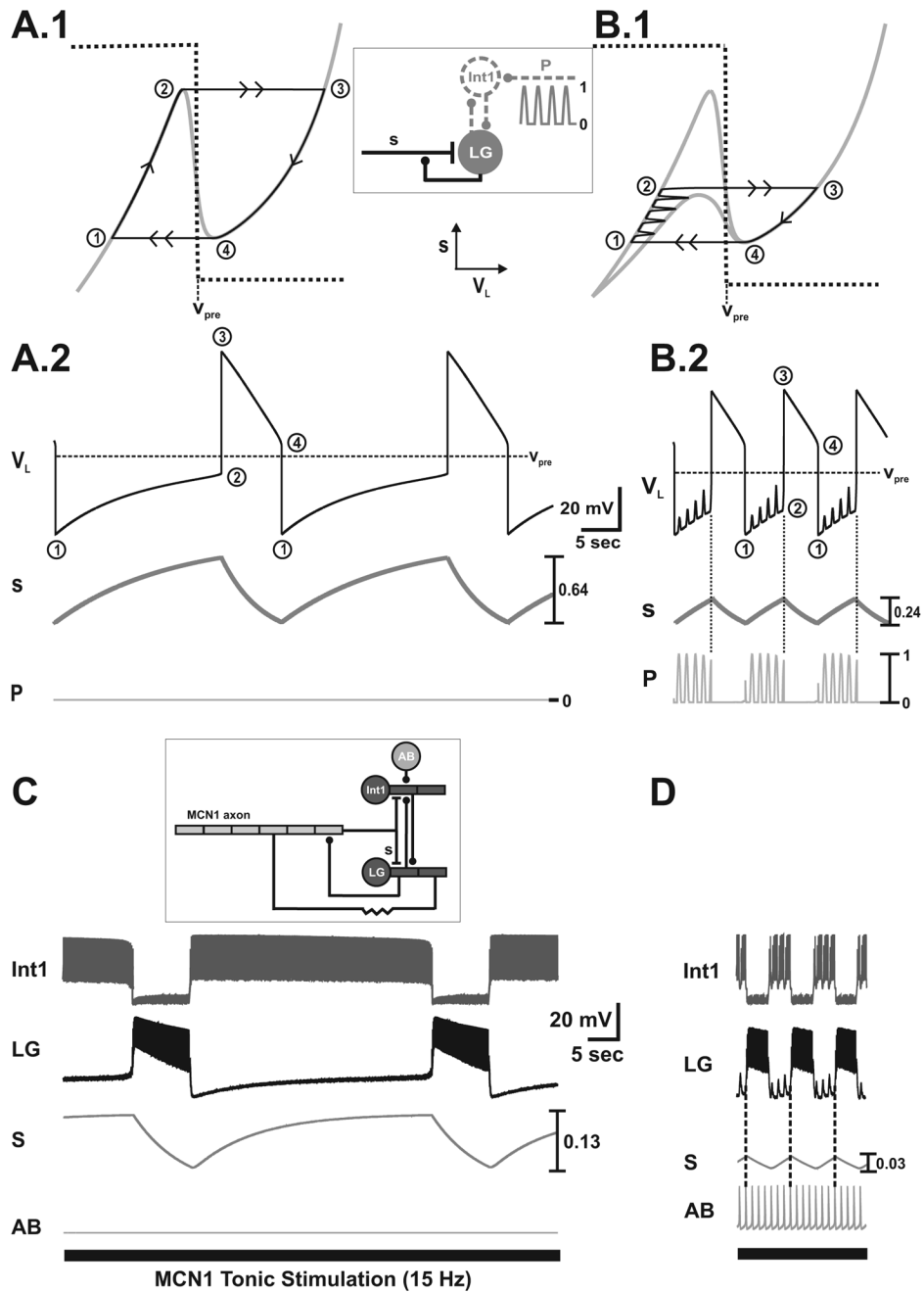
Figure 2. The buildup and decay of MCN1 excitation ( s ) in the LG neuron drives the MCN1-elicited gastric mill rhythm. A.1-A.2 , Network dynamics in the absence of pyloric input ( p = 0 ). During the inactive state of the LG neuron, the trajectory slowly climbs up the left branch of the V_L -nullcline from point 1 to point 2 ( A.1 ), and s builds up in the LG neuron as the LG membrane potential ( V_L ) slowly rises ( A.2 ). At point 2 the trajectory jumps to point 3 on the right branch of the cubic, since dV_L/dt > 0 above the V_L -nullcline. During the active state of the LG neuron, the trajectory slowly falls down the right branch of the V_L -nullcline from point 3 to point 4 ( A.1 ) due to LG presynaptic inhibition of MCN1, and s decays in the LG neuron as V_L slowly falls ( A.2 ). At point 4, the trajectory jumps back to point 1 on the left branch of the cubic, since
