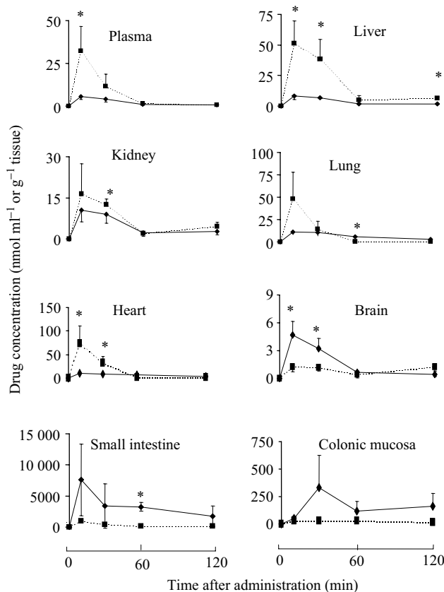
Figure 3 Concentrations of resveratrol (squares, dotted line) and DMU 212 (rhombi, solid line) in the plasma and tissues of mice that received a single dose of drug ( 240\text{ mg kg}^{-1} ) i.g. Values are the mean \pm s.d. ( n=3 ). Star indicates that the values differ significantly ( P<0.05 , one-way ANOVA). For details of dosing, extraction and HPLC analyses, see Materials and Methods.
