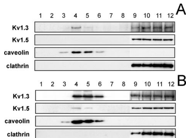
FIGURE 7. Activation of macrophages targets Kv1.5 back to lipid rafts. Detergent-based isolation of lipid rafts from bone marrow derived macrophages cultured in the absence ( A ) or the presence ( B ) of 100 ng/ml LPS. Sucrose density gradient fractions were analyzed by Western blot. Although caveolin localized low buoyancy raft fractions, clathrin marked nonfloating fractions. LPS increased the relative abundance of Kv1.3 ( 12 \pm 2 and 40 \pm 3\% , for control and LPS-treated cells, respectively; p < 0.01 , Student's t test) and shifted Kv1.5 to low buoyancy rafts ( 10 \pm 1\% in LPS-treated cells) in macrophages. The values are the means \pm S.E. of four independent experiments.
