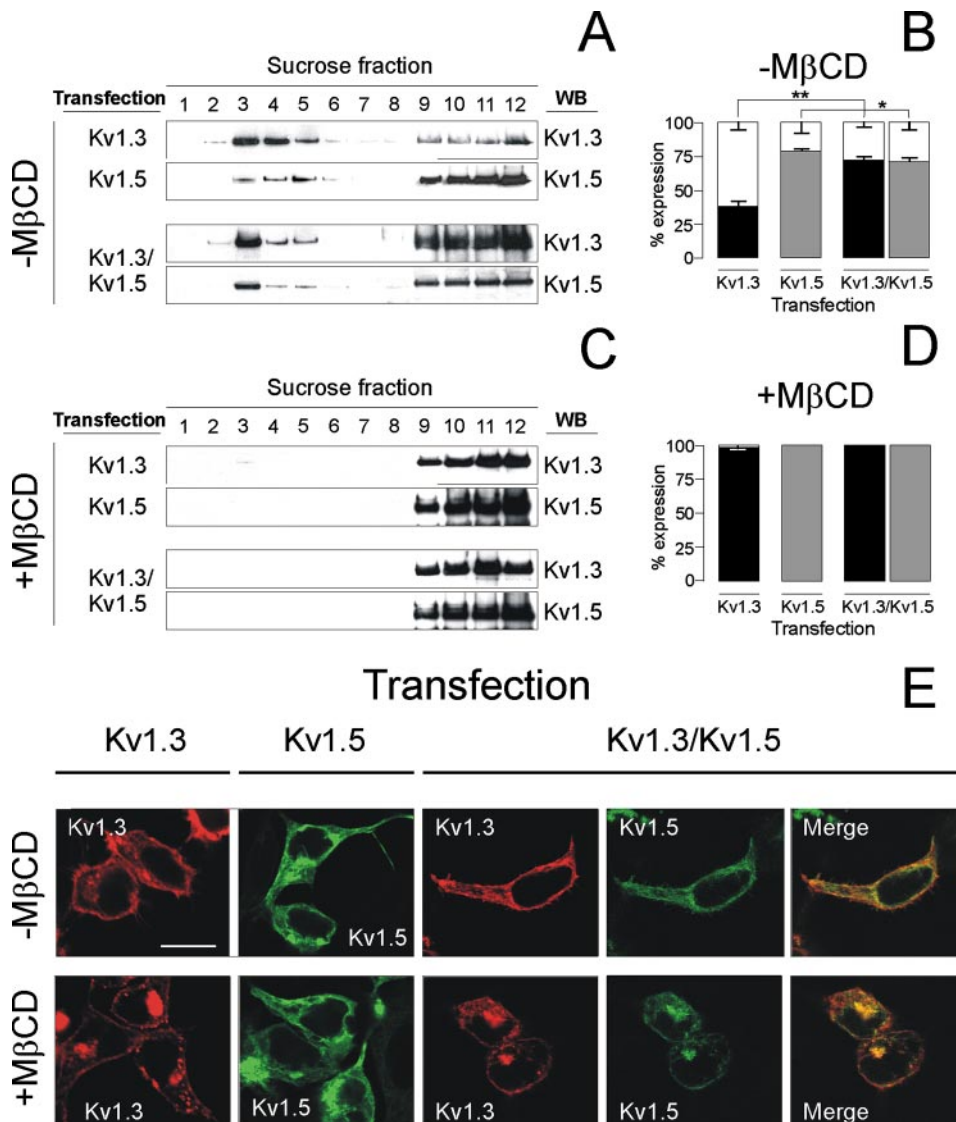
FIGURE 4. Cholesterol depletion impairs Kv1.3, Kv1.5, and Kv1.3/Kv1.5 localization in lipid rafts. HEK cells were treated with or without 2% M \beta CD 1 h before lipid raft extraction (A–D) and confocal microscopy studies (E). A and C, cells were transfected with Kv1.3, Kv1.5, and Kv1.3/Kv1.5 (ratio 1:1) and fractions immunoblotted (WB) against the channels. B and D, quantification of data from A and C. Relative abundance (%) of the protein expression located in floating (white bar) and nonfloating (black bar, Kv1.3; gray bar, Kv1.5) fractions. 100% represents the overall protein expression in all fractions. The values are the means \pm S.E. of four independent experiments. *, p < 0.05 ; **, p < 0.01 (Student's t test). A and B, cells incubated without M \beta CD (–M \beta CD). C and D, cells incubated with M \beta CD (+M \beta CD). E, M \beta CD did not alter Kv1.3, Kv1.5, and Kv1.3/Kv1.5 expression patterns. The cells were transfected as described above and incubated in the absence (top panels, –M \beta CD) or the presence (bottom panels, +M \beta CD) of M \beta CD. HEK cells were transfected with Kv1.3-YFP (red), Kv1.5-CFP (green), and both (Kv1.3/Kv1.5). The merge panels show colocalization (yellow) in doubly transfected cells. The bars represent 10 \mu m.
