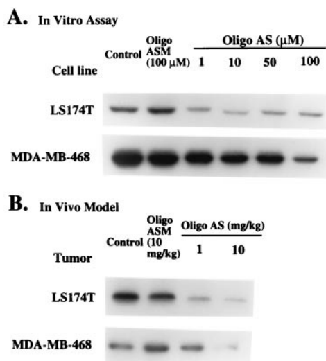
Fig. 1. (A) Effects of oligos on the expression of the RI \alpha subunit of PKA in LS174T and MDA-MB-468 cells. Cultured cells were treated with Oligo AS or ASM at various concentrations for 24 h. Identical amounts of total protein (50 \mu g) were fractionated by SDS/PAGE and analyzed by Western blotting. For LS174T cells, at the concentrations of 1 and 10 \mu M, Oligo AS inhibited RI \alpha subunit expression by about 80%, with no significant dose–response being observed at higher concentrations. For MDA-MB-468 cells, a significant dose–response relationship was observed. At the highest concentration, Oligo AS inhibited the RI \alpha subunit expression by about 75%. In contrast, Oligo ASM had no effect on RI \alpha subunit expression for either cell line. (B) Effects of oligos on the expression of the RI \alpha subunit of PKA in LS174T and MDA-MB-468 tumor xenografts. Animals with LS174T xenografts were treated with oral administration of Oligo AS or ASM for 1 week. Animals with MDA-MB-468 xenografts were treated with oral administration of Oligo AS or ASM for 6 weeks. Identical amounts of total protein (100 \mu g) from the tumor homogenates were used in Western blot analysis. A dose-dependent inhibition of the RI \alpha subunit expression was observed in both tumor models. At 10 mg/kg, Oligo AS inhibited RI \alpha subunit expression by about 80%. In contrast, Oligo ASM had no effect.
