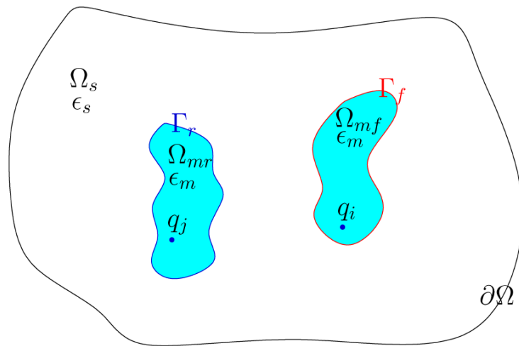
Fig. 1. Illustration of macromolecules immersed in aqueous solvent environment.
