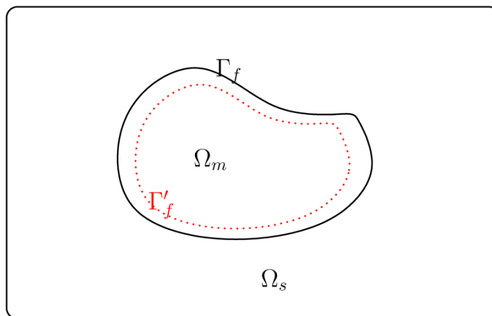
Fig. 2. Displacement of the molecular surface \Gamma_f . The solid black line is the surface before displacement and the dashed red line is the surface after displacement. The new solvent region \Omega'_s is \Omega_s plus the strip between two surfaces; The strip subtracted from \Omega_m equals the new solute region \Omega'_m .
