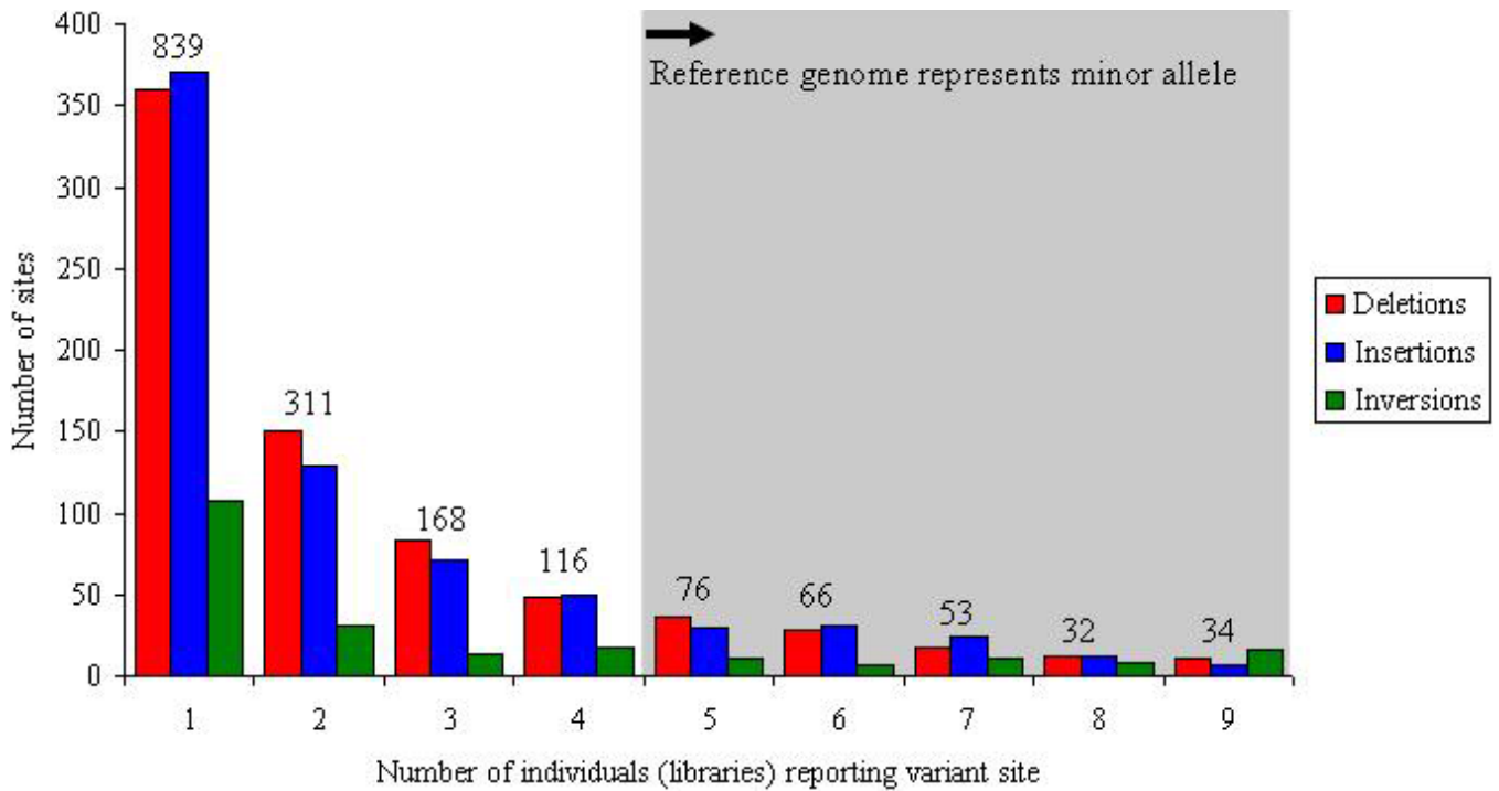
Figure 2. Frequency distribution
