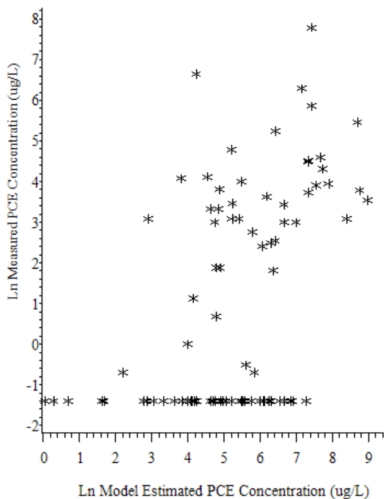
Figure 1 Log e measured PCE versus log e model estimated PCE concentrations (ug/L).
