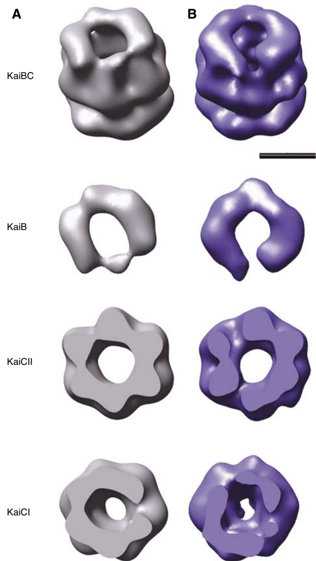
Figure 4 Negative-stain EM structures of the SeKaiBC complex. (A) Three-dimensional reconstruction of the KaiBC complex based on 7415 particle images (selected from the total dataset of 8720) processed without imposed symmetry. The full reconstruction (top) and its three density layers assigned to KaiB, the ring of KaiC CII domains and the ring of KaiC CI domains are shown. (B) Three-dimensional reconstruction of the KaiBC complex based on 1106 particle images (selected from a sub-dataset of 1880 grouped with the model containing two parallel KaiB dimers) processed without imposed symmetry. Both structures have a resolution of 19\text{ \AA} and are shown filtered to 19\text{ \AA} resolution. The isosurface values are set to enclose 100% of the expected volume for a KaiC hexamer and two KaiB dimers. The scale bar represents 50\text{ \AA} .
