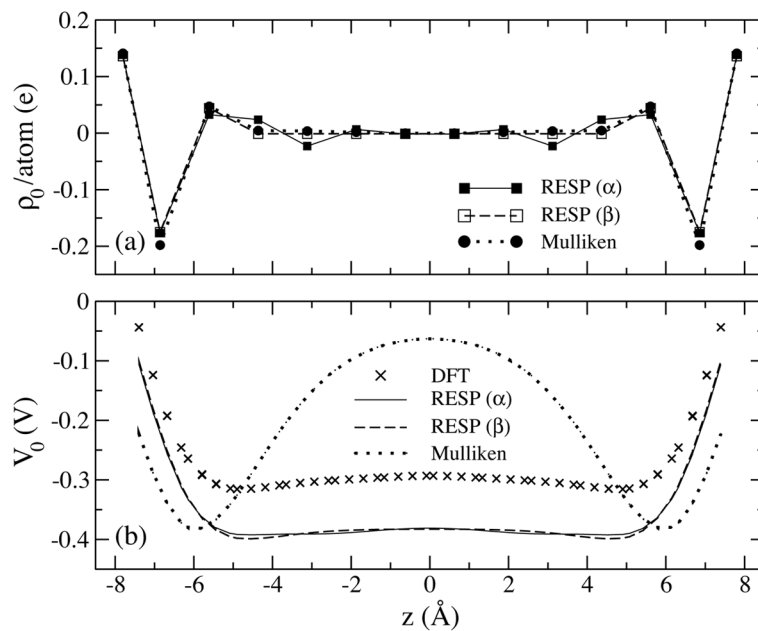
Figure 2. (a) Atomic partial charges determined from RESP (model \alpha and \beta ) and Mulliken population analysis for a (6,6) SWNT segment of 12 sections. (b) Corresponding electrostatic potential along the tube axis in comparison with results from DFT calculations.
