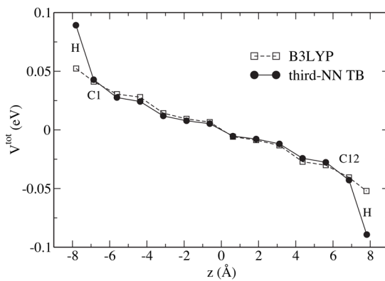
Figure 4. Total electrostatic potential on a (6,6) SWNT segment with 12 sections in a uniform axial field of strength E = 25.7\text{mV}/\text{Å} .
