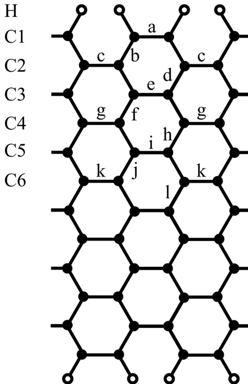
Figure 1. Schematic view of a 12-section armchair SWNT. Carbon atoms are shown as solid circles and hydrogen atoms as open circles.
