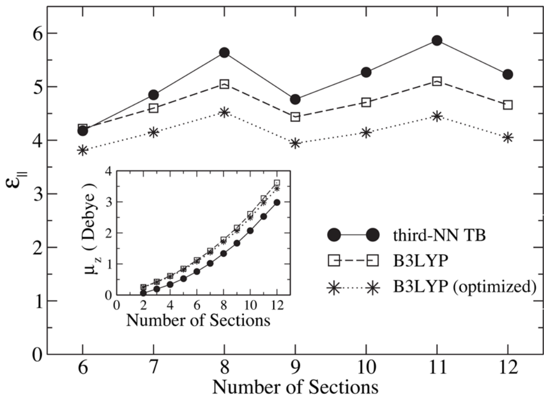
Figure 5. Parallel dielectric constant, \epsilon_{||} , for (6,6) SWNT segments with 6–12 sections. Inset: Induced dipole moment under a parallel field of E = 25.7 \text{ mV/\AA} as a function of SWNT length.
