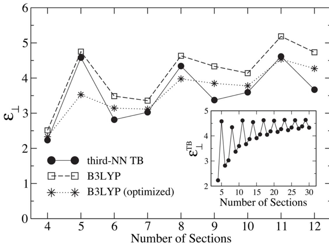
Figure 7. Dielectric constant \epsilon_{\perp} for (6,6) SWNT segments with 4–12 sections. Inset: Third-NN TB dielectric constant, \epsilon_{\perp}^{TB} , for SWNTs with up to 30 sections.
