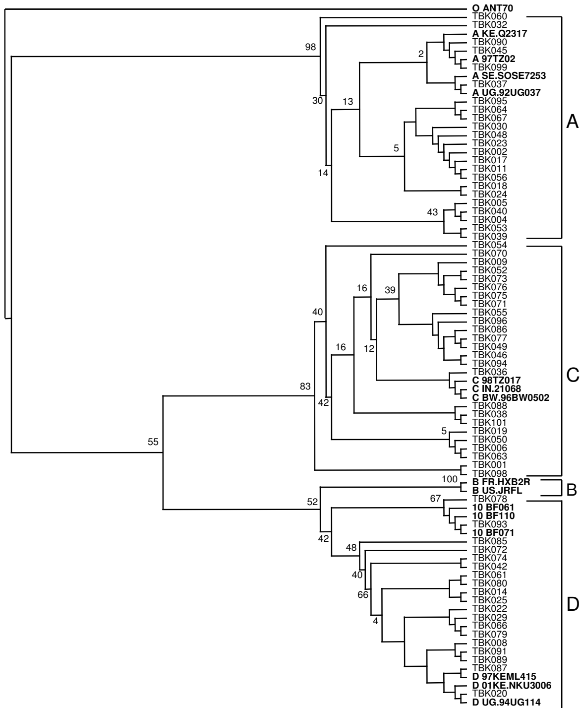
Figure 2 Phylogenetic analysis of HIV-1 pol sequences from HIV-1 infected pregnant women in Bukoba, Kagera. The study and reference sequences were aligned by the Cluster X programme and tree constructed by neighbour-joining method based on the Kimura two-parameter and viewed using TreeView software. Sequence O ANT70 was used as out-group for phylogenetic analysis.
