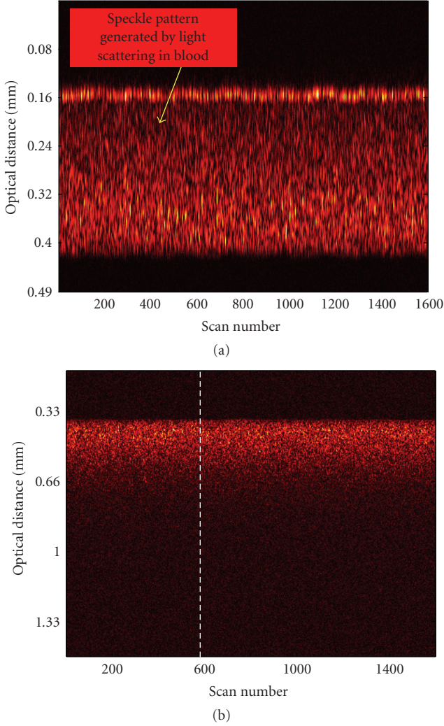
FIGURE 1: (a) OCT image of blood flowing through the 0.2-mm cell. Both blood/glass interfaces are visible. (b) OCT image of blood flowing through the 2-mm cell. The interrupted white line marks the 600th A-scan. Both images are composed of 1600 A-scans.
