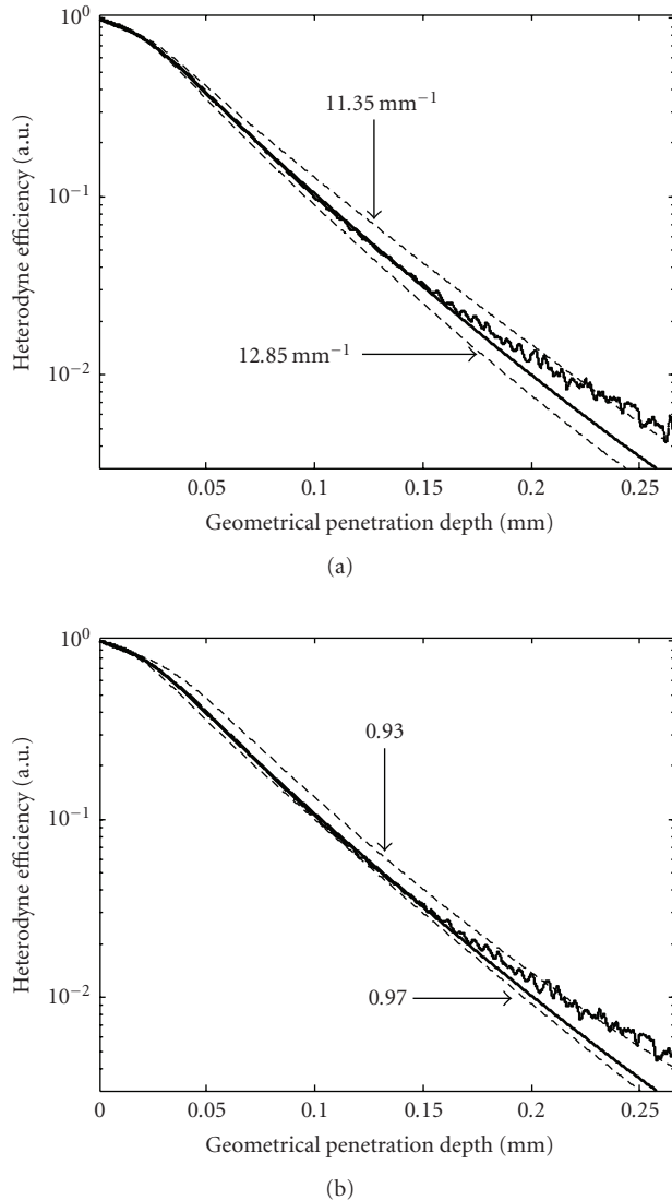
FIGURE 3: Best numerical fit with the experimental heterodyne profile is obtained for values of \mu = 12.15 \text{ mm}^{-1} and g = 0.95 for the attenuation coefficient and anisotropy parameter, respectively. The numerical fit is the middle line that follows closely the experimental heterodyne efficiency curve shown in both (a) and (b) parts of the figure. (a) Variations of the numerical fit induced by changes of \pm 0.7 \text{ mm}^{-1} in the attenuation coefficient with the anisotropy scattering factor kept at g = 0.95 . (b) Variations in the numerical fit induced by variations of \pm 0.02 in the scattering anisotropy parameter with the attenuation coefficient kept at \mu = 12.15 \text{ mm}^{-1} .
