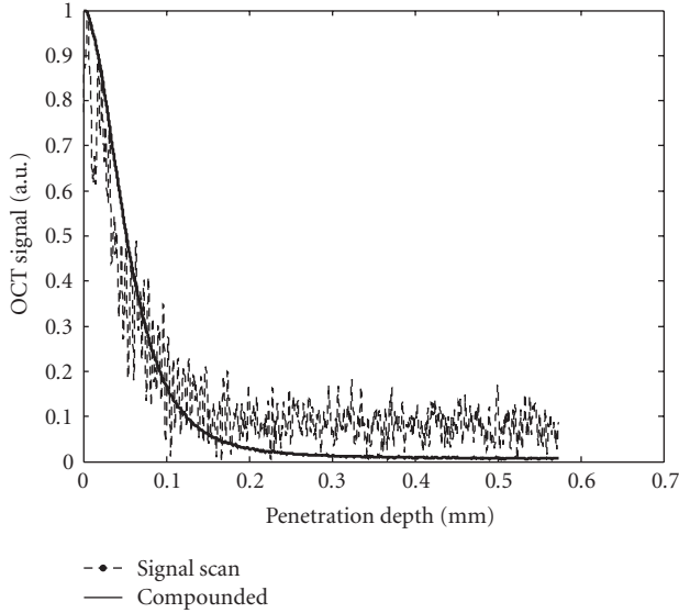
FIGURE 2: Single OCT depth-line scan (dotted line) compared to the compounded profile (continuous curve). The single-scan line is the 600th A-scan marked with a white interrupted line in Figure 1(b). The compounded profile results from the summation of 1000 consecutive A-scans.
