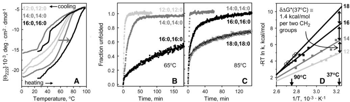
Fig. 4. Effect of acyl chain length on thermal denaturation of apoC-I complexes with fully saturated phosphatidylcholines (PCs). Discoidal complexes of apoC-I (20 \mu\text{g}/\text{ml} protein in 5 mM Na phosphate, pH 7.7) with dilauroyl PC (DLPC) (light gray), dimyristoyl PC (DMPC) (gray), dipalmitoyl PC (DPPC) (black), or distearoyl PC (DSPC) (black open symbols) in 5 mM \text{NaH}_2\text{PO}_4 , pH 7.7, were used. A: CD heating and cooling data, \Theta_{222}(T) , recorded at a scan rate of 11°C/h (the data for DSPC are not shown to avoid overlap). Shift in the heating curves upon increase in the acyl chain length is shown by the gray arrow. The hysteresis between the heating and cooling curves was addressed earlier (16, 17) and is a hallmark of a kinetically controlled transition with high free energy barrier for forward and reverse reaction. The hysteresis is reduced for shorter-chain DLPC, reflecting relative ease of spontaneous protein reconstitution with this lipid. B, C: Kinetic CD data, \Theta_{222}(T) , recorded in T-jumps to 65°C or 85°C (for complexes with PCs containing 12–16 or 14–18 carbons, respectively). The data are normalized to fraction unfolded (D) Arrhenius plots for apoC-I complexes with PCs differing in chain length. The plot for each complex was obtained from exponential approximation of the T-jump data such as those in Fig. 2A; for DPPC- and DSPC-containing particles, the first kinetic phase corresponding to disk fusion is shown. Linear extrapolation of the Arrhenius plots to 37°C (solid lines) suggests that increasing chain length by two \text{CH}_2 groups increases the kinetic disk stability by approximately 1.4 kcal/mol (double arrows).
