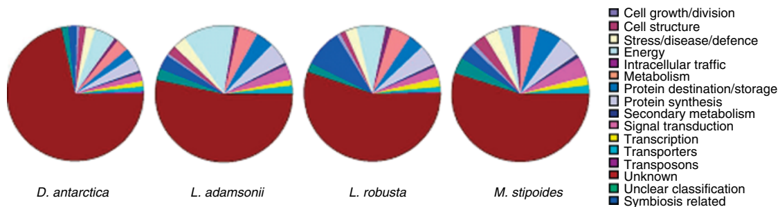
Figure 2. Distribution of functional categories amongst EST clusters in xenogenomics target species
