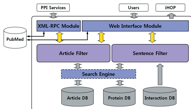
Figure 1. Overview of PIE. The PIE system consists of several modules. 'Article Filter' and 'Sentence Filter' decide whether given articles or sentences contain PPI information. 'Search Engine' retrieves the stored information such as learning data (Article DB) and protein names (Protein DB). 'Interaction DB' means the database including interaction-related words. 'XML-RPC Module' is responsible for RPC communication with other PPI services. 'Web Interface Module' manages the whole process of PPI predictions from Web users. Prediction results contain the links to the iHOP service to provide further protein information. For PubMed search, PIE retrieves PubMed articles using the NCBI E-Utilities.
