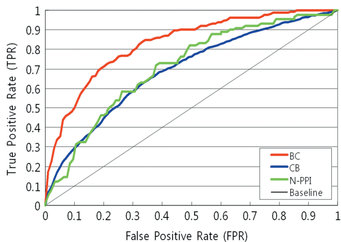
Figure 3. ROC curves for test data. Performance of PIE has been measured using independent test sets. The options on PIE was set to using simplified tags and protein dictionary. In all cases, TPR is rapidly increased at low FPR, implying that the system performs high precision predictions for high-probability sentences.
