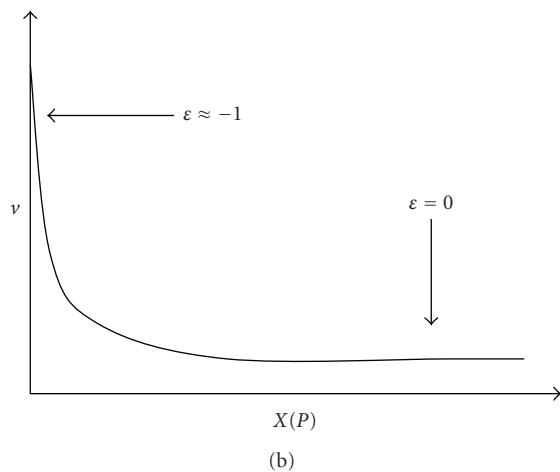
FIGURE 6: Elasticity coefficients.
