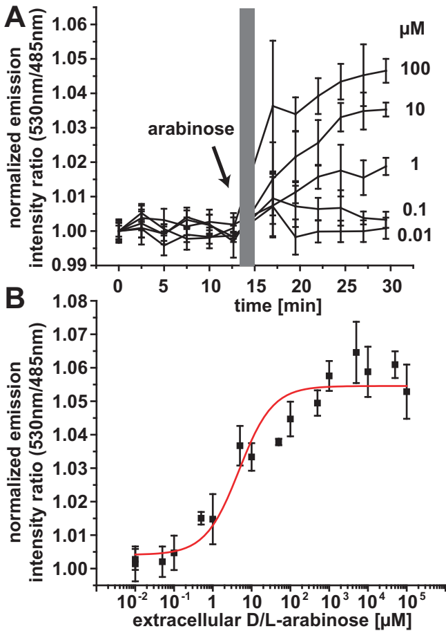
Figure 3 Detection of intracellular arabinose with FLIPPara-200n. (A) Detection of intracellular arabinose in Escherichia coli BL21-Gold(DE3) cells expressing FLIPPara-250n. The arrow indicates arabinose addition (note that here the addition was performed by hand, leading to an interruption of the protocol, thus rates cannot be deduced; marked as a gray bar). Error bars indicate the standard deviation of at least three replicates. (B) Arabinose-dependent sensor in vivo response at t = 25 minutes. The intracellular arabinose concentration that corresponds to the affinity constant ( K_d ) of FLIPParaF.Ec-250n is reached at an external arabinose concentration of 4.7 \pm 2.0 \mu\text{M} , indicating that the intracellular concentration is around 20-fold lower compared with the extracellular concentration in a medium containing 4.7 mM arabinose. Error bars represent the standard deviation ( n = 3 ).
