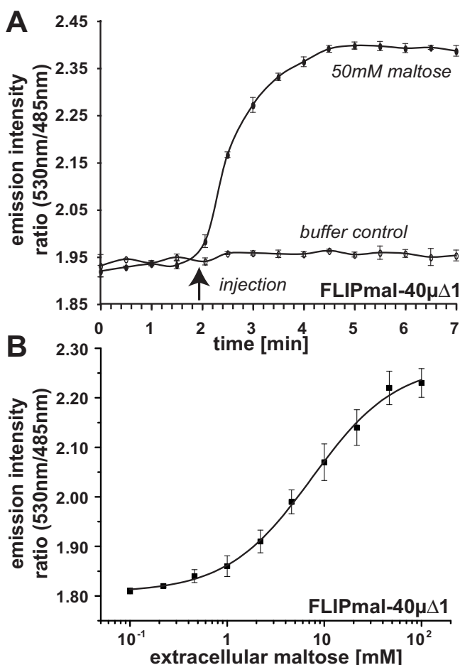
Figure 5 Accumulation of intracellular maltose detected with FLIPmal sensors. (A) Cytosolic maltose accumulation measured in 30-second intervals after injection of buffer or 50 mM maltose to microtiter plate wells containing Escherichia coli BL21-Gold(DE3) cells expressing FLIPmal-40 \mu\Delta -enhanced yellow fluorescent protein. The arrow indicates the time point of maltose addition using the injector of the Tecan Infinite M200 fluorimeter (note, in contrast to Figure 3A, this procedure allows the determination of rates). (B) Dose-response curve for maltose detected by FLIPmal-40 \mu\Delta -enhanced yellow fluorescent protein in E. coli BL21-Gold(DE3) cells. Intracellular maltose levels are around 700-fold lower compared with the external concentration ( K_{0.5} = 7.4 mM). Error bars represent the standard deviation ( n = 3 ).
