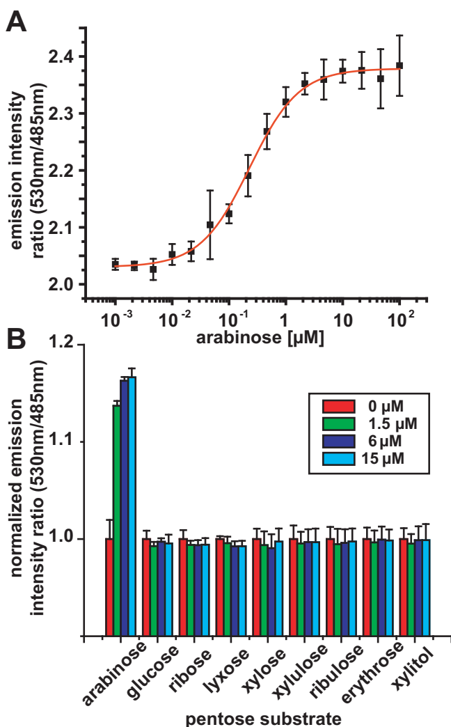
Figure 2 In vitro analysis of the arabinose nanosensor FLIPara-200n. (A) In vitro Venus/enhanced yellow fluorescent protein ratio change of affinity-purified FLIPara-250n in the presence of D/L-arabinose. The binding constant K_d of the sensor is 230 \pm 18 nM (derived from single-site binding isotherm fit). (B) Substrate specificity of FLIPara-250n as measured by fluorescence resonance energy transfer in the presence of various pentose ligands at three different concentrations. Data were normalized to the sensor in the absence of ligand (first bar on left). Error bars represent the standard deviation ( n = 3 ).
