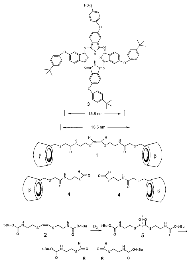
Scheme 1. Structures and the cleavage reaction.
