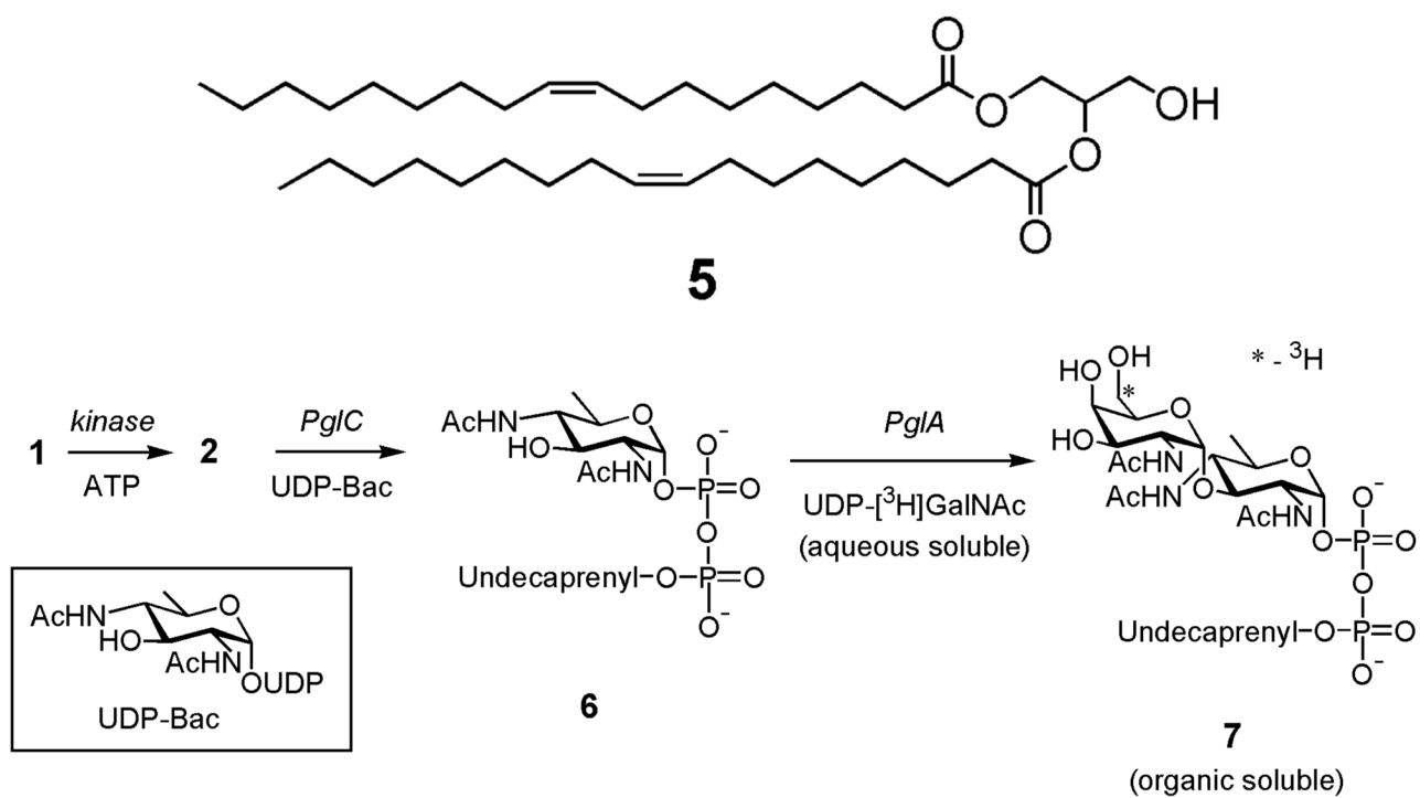
Figure 3. An enzymatic reaction scheme showing the synthesis of undecaprenyl pyrophosphate-linked disaccharide ( 7 ).
