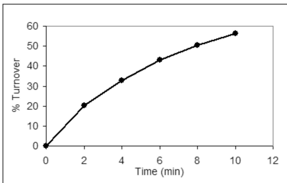
Figure 6. A time course of a PglB reaction in which radiolabeled undecaprenyl pyrophosphate disaccharide is used as a substrate.
