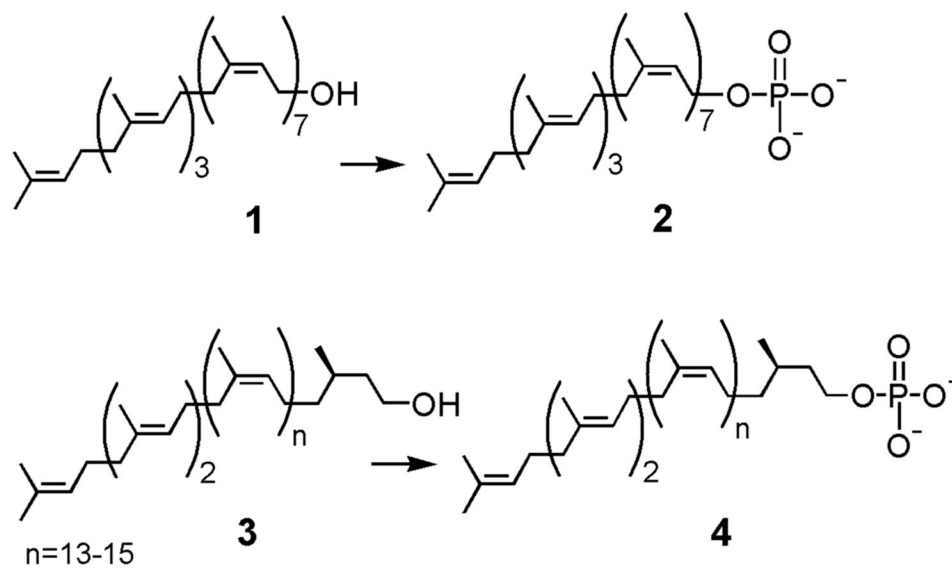
Figure 2. Undecaprenol (1) and dolichol (3) can be phosphorylated to form undecaprenyl phosphate (2) and dolichyl phosphate (4), respectively. This reaction can be done synthetically or chemoenzymatically by the action of a kinase.
