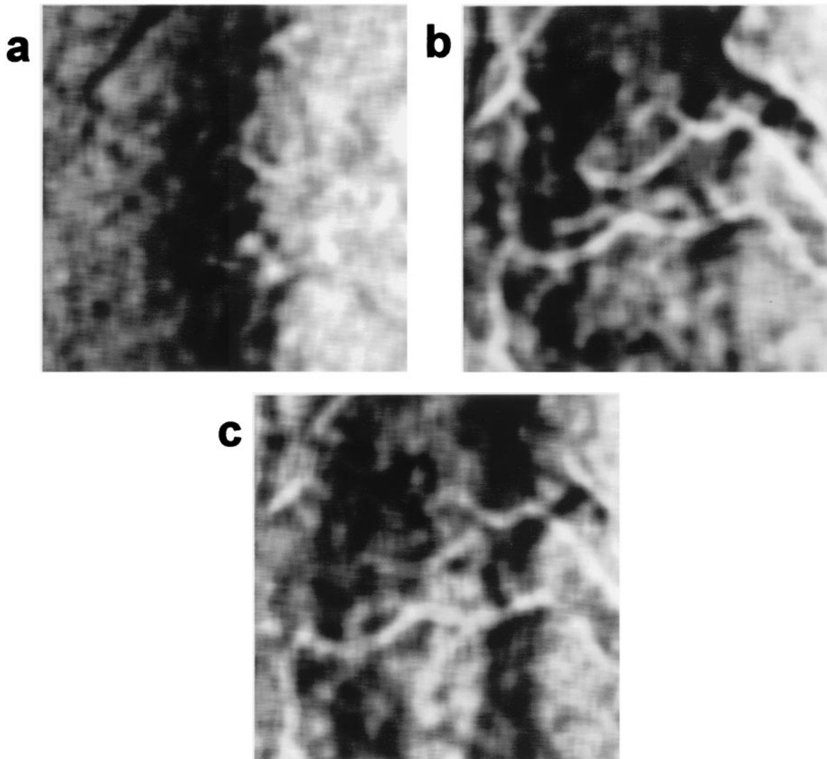
Fig. 3. Demonstration of perception-specific signals using illusory stimuli in the same patch of cortex. (a) A visual target with a width of 0.12^\circ and 102^\circ orientation. (b) Response to a masking stimulus presented alone. (c) Response to the target and mask presented together as the “standing wave of invisibility.” Notice that the representation of the target seen in a is now missing, just as it is invisible perceptually.
