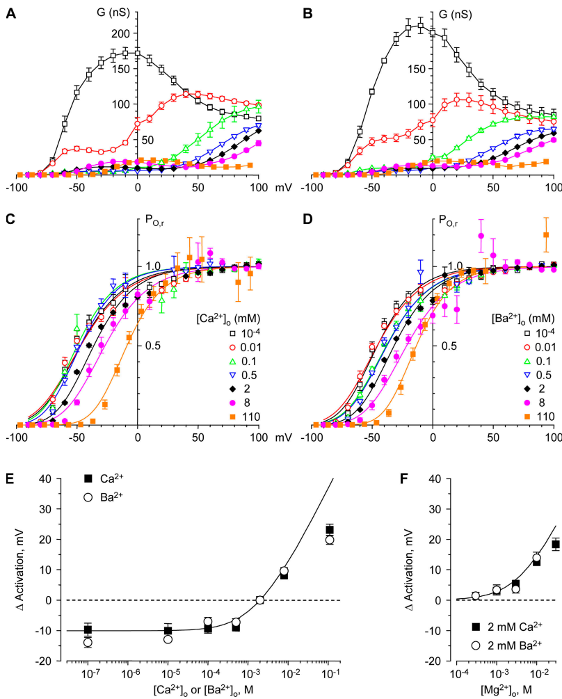
Figure 11. Effects of Ca 2+ o , Ba 2+ o , and Mg 2+ o on gating. (A and B) Chord conductances; (C and D) channel activation. Activation was measured as the relative channel open probability (P O,r ) from the I-V/IIV ratio, normalized (see Materials and methods). Smooth curves in C and D are fits to fourth power Boltzmann relationships. (E and F) Shifts in activation with Ca 2+ o or Ba 2+ o (E) and Mg 2+ o (F). Data are from Fig. S8 A (Ca 2+ o and Ba 2+ o ) and Fig. S16 A (Mg 2+ o ), except that voltage shifts in Ba 2+ o are defined with respect to 2 mM Ba 2+ o (not 2 mM Ca 2+ o ). The smooth curve is the fit to Gouy-Chapman theory with a single uniform surface charge density (see Materials and methods).
