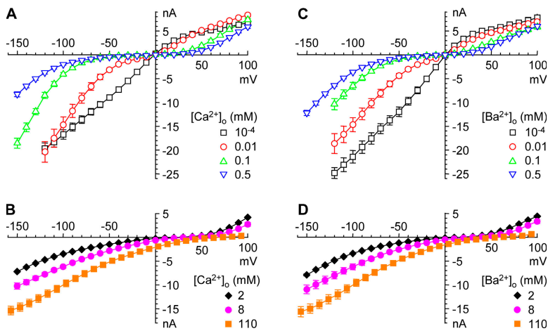
Figure 2. I-V relations at different concentrations of \text{Ca}^{2+}_o (A and B) and \text{Ba}^{2+}_o (C and D). Values are from 5, 8, 5, 7, 4, and 3 cells in \text{Ca}^{2+}_o , and 3, 5, 7, 6, 4, and 3 cells in \text{Ba}^{2+}_o (respectively, 100 nM, 10 \mu\text{M} , 0.1 mM, 0.5 mM, 8 mM, and 110 mM). Control values at 2 mM \text{Ca}^{2+}_o or \text{Ba}^{2+}_o are averaged from all these cells (32 in \text{Ca}^{2+}_o , 28 in \text{Ba}^{2+}_o ). In each cell, the control value was the average of measurements before and after the test solution, to correct for rundown. Values were normalized for each cell as described in Materials and methods. Figs. 3–5 are based on this same dataset.
