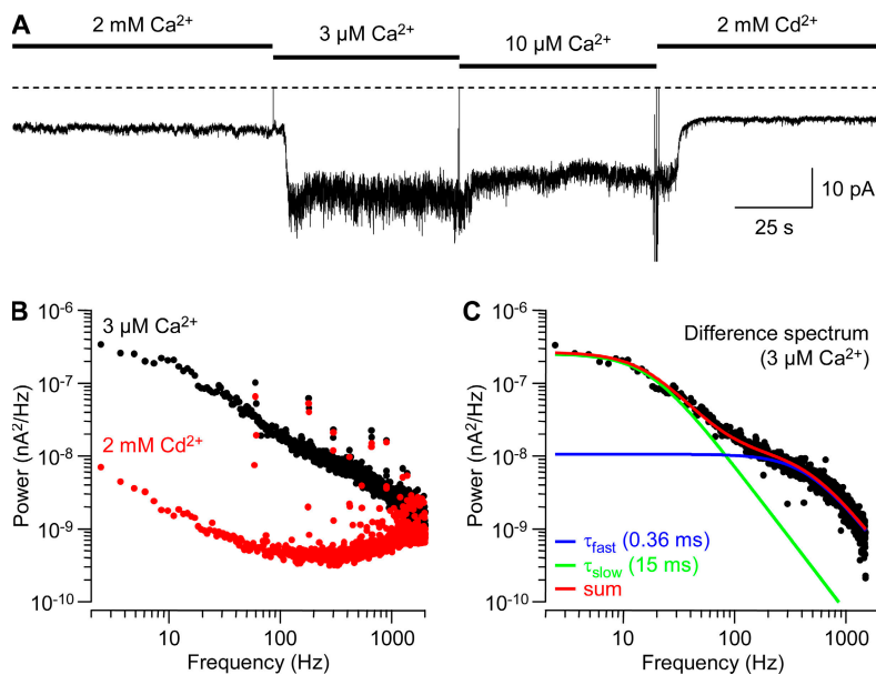
Figure 7. Noise analysis of block by Ca 2+ o . (A) “Window” currents at -60 mV in 2 mM, 3 \mu M, and 10 \mu M Ca 2+ o ; and in 2 mM Cd 2+ o . 8-pole analogue Bessel filter at 2 kHz. (B) Averaged power spectra in 3 \mu M Ca 2+ o and 2 mM Cd 2+ o , from \sim 60-s records analyzed in 819.2-ms segments, using a Hamming window. (C) The difference between the spectra shown in B, fitted to the sum of two Lorentzian components (440 and 10.5 Hz, corresponding to time constants of 0.36 and 15 ms).
