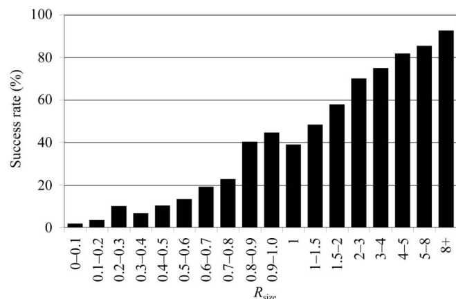
Figure 10 Efficiency of the identification of the binding site in the presence of other smaller ( R_{\text{size}} > 1 ) or larger ( R_{\text{size}} < 1 ) ligands.
