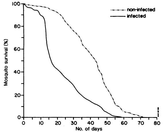
Fig. 3. Cumulative daily survival rate of non-infected mosquitos and of mosquitos infected with mean number of oocysts >71.
