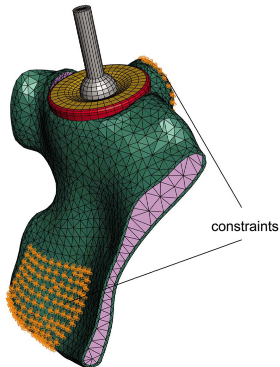
Fig. 6. Constraints of the Models A and B, simulation of the constraint conditions of the hip simulator (a) and the constraint conditions of the bovine bone Model D (b)
