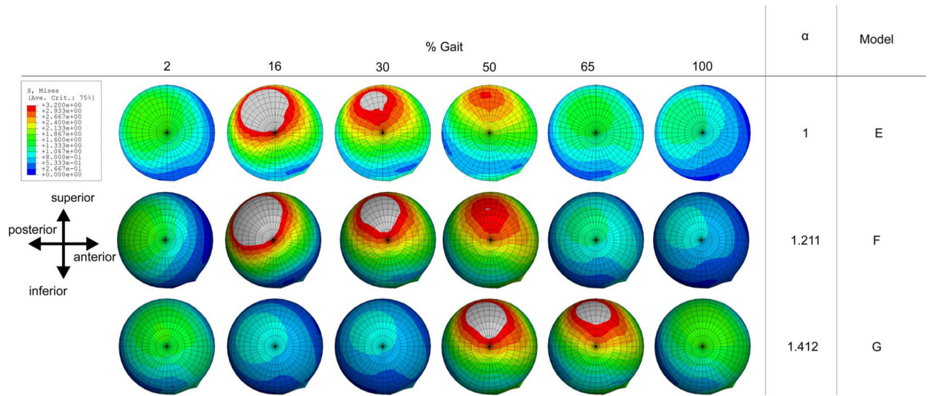
Fig. 8. Comparison of von Mises stresses in the cement mantle near the bone-cement interface under normal walking (E), ascending stairs (F), and descending stairs (G) loading conditions
