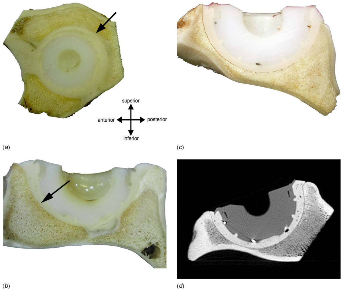
Fig. 9. Results from the preliminary hip simulator tests. (a) Partial failure in the posterior-superior quadrant at the bone-cement interface (normal walking, 15 \times 10^6 cycles, BW 100 kg); (b) multiple discrete failures at the bone-cement interface (normal walking, 17 \times 10^6 cycles, BW 100 kg); (c) near-complete failure at the bone-cement interface (descending stairs, 2.2 \times 10^6 cycles, BW 125 kg); (d) a CT scan image showing extensive radiolucent line at the bone-cement interface of sample shown in (c).
