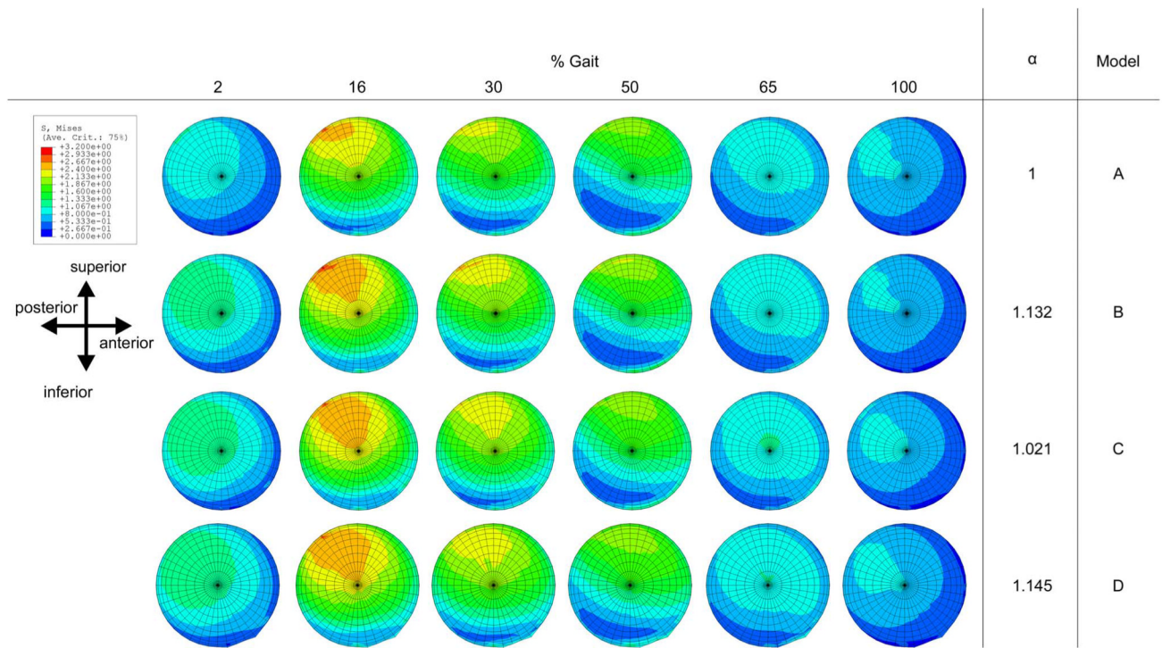
Fig. 7. A summary of von Mises stresses in the cement mantle near the bone-cement interface from selected FE models
