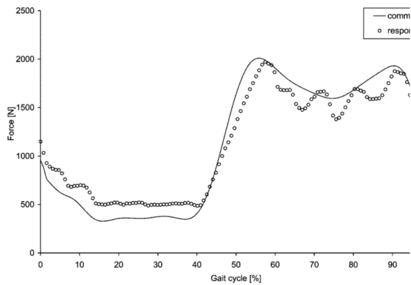
Fig. 4. Comparison of the hip contact forces as demand signal (line) and response of the machine (symbol) for normal walking (a), ascending stairs (b), and descending stairs (c)
