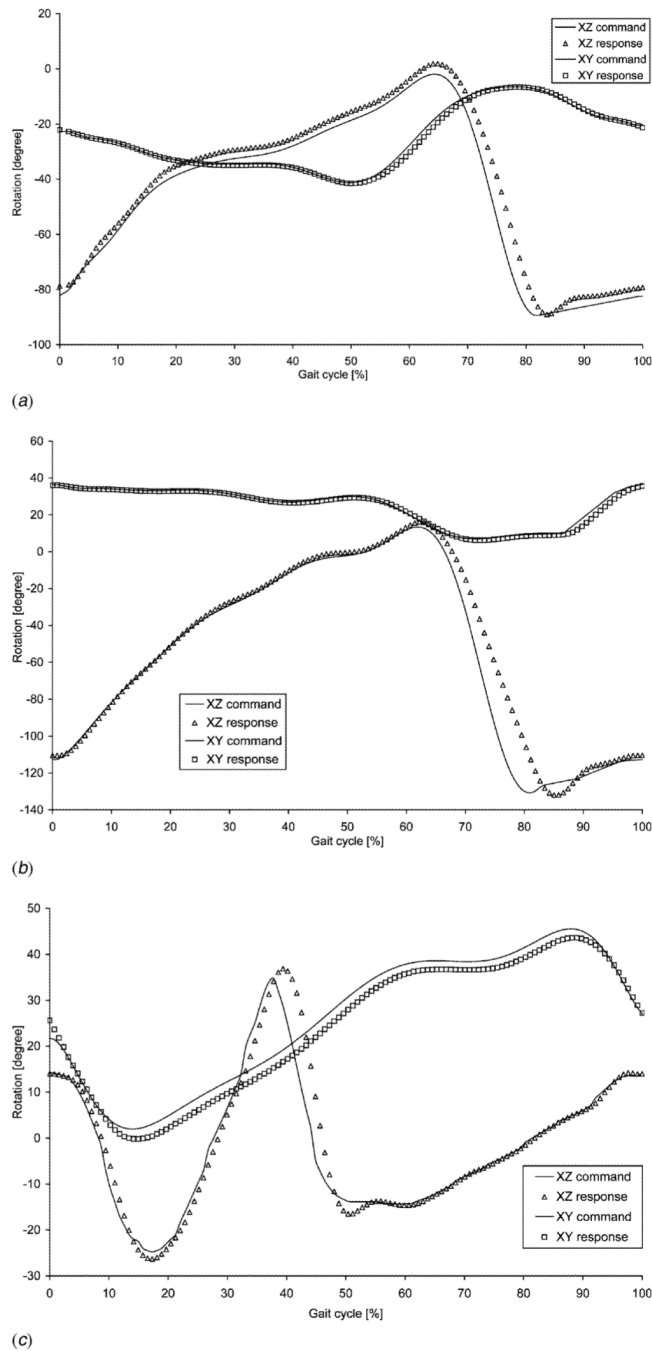
Fig. 5. Comparison of the motions as demand signal (line) and response of the machine (symbol) for normal walking (a), ascending stairs (b), and descending stairs (c)
