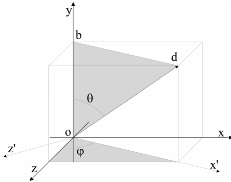
Fig. 1. The resultant hip contact force relative to the cup coordinate system. Note that the magnitude and the orientation of the hip contact force may be achieved by two rotary actuators about y and z' axes, respectively. z' is perpendicular to the obd plane. The rotations are represented by angle \varphi and \theta .
