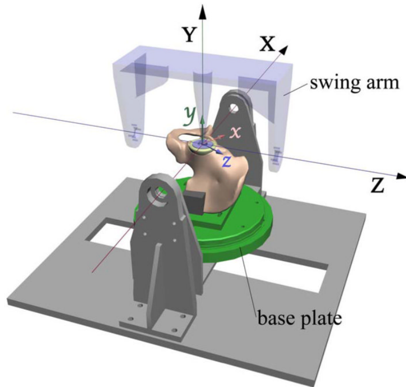
Fig. 2. Schematic diagram of the motions of the Portsmouth hip simulator with the coordinate systems shown in the machine frame ( X, Y, Z ) and cup frame ( x, y, z ), as used by Bergmann et al. [12]
