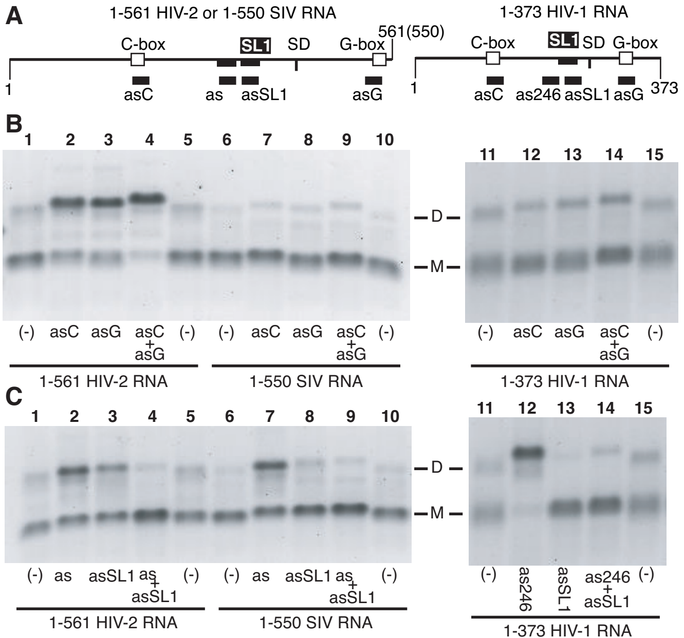
Figure 3 Antisense oligonucleotide-mediated activation or suppression of HIV-2, SIV and HIV-1 RNA tight dimerization. A. Schematic representation of the leader RNAs as described in Figure 1 with the oligonucleotide binding sites indicated (left panel, HIV-2 or SIV, right panel, HIV-1). B. 1-561 HIV-2 (left), 1-550 SIV (center) and 1-373 HIV-1 (right) RNAs were incubated at 55°C for 30 minutes in their respective dimer buffers with or without a 20-fold molar excess of antisense oligonucleotides directed against the C-box or G-box elements (Table 2) before loading on a TBE/26°C agarose gel. The 5' end of all asG oligonucleotides bind to the start codon of the gag gene in the G-box element and thus to the majority of nucleotides involved in the CGI structures (8 nts out of 13, Figure 1F). The asC oligonucleotides bind to all (HIV-2 and SIV) or most (HIV-1, 10 nts out of 13) of lentiviral C-box elements (Figure 1F). Lanes 1, 5, 6, 10, 11 and 15 correspond to RNA incubated in dimer buffer at 55°C without oligonucleotide. The monomer and dimer RNA species are indicated by M and D, respectively. C. 1-561 HIV-2 (left), 1-550 SIV (center) and 1-373 HIV-1 (right) RNAs were incubated at 55°C for 30 minutes in dimer buffer with or without a 20-fold excess of antisense oligonucleotides directed against sequences upstream of SL1 and including stem B (asΨ in HIV-2 and SIV, as246 in HIV-1) or the loop and 5' stem of SL1 (asSL1) before loading on a TBE/26°C agarose gel.
