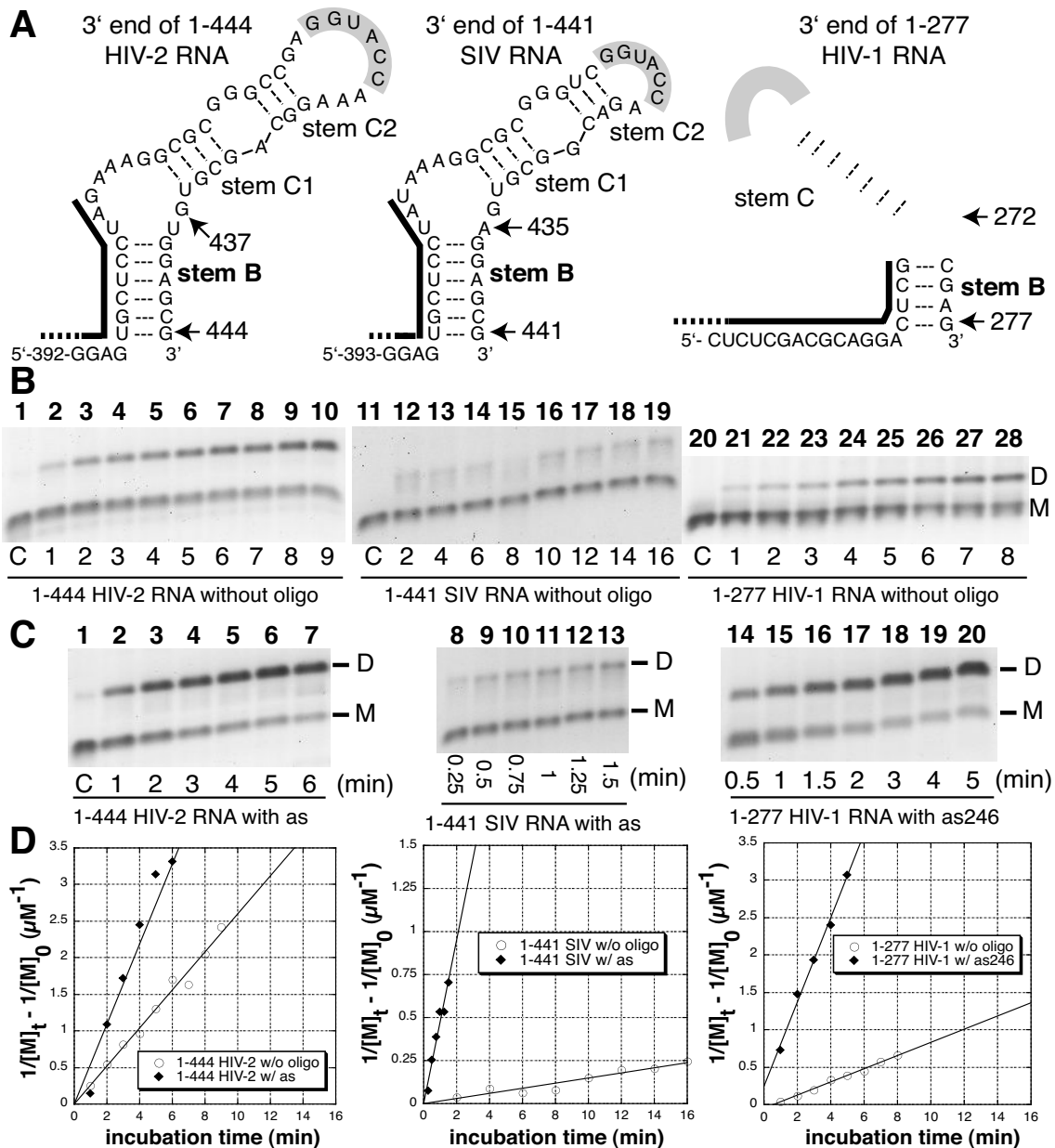
Figure 5 Anti-stem B oligonucleotide-mediated activation of HIV-2, SIV and HIV-1 RNA tight dimerization. A. Schematic representation of HIV-2, SIV, and HIV-1 SLI domains. The black bars represent the binding sites of antisense oligonucleotides used in this experiment (Table 2). B and C. The time-dependent dimerization of 1-444 HIV-2, 1-441 SIV and 1-277 HIV-1 RNAs were measured at 55°C as described in Figure 4, without (B) or with (C) a 20-fold excess of antisense oligonucleotides directed against the sequence upstream of SLI including the 5' side of stem B (A and Table 2). Typical kinetics experiments with 1-444 HIV-2 RNA (B and C, left panels), 1-441 SIV SLI (B and C, middle panels), and 1-277 HIV-1 RNA (B and C, right panels) are shown. Lanes I (B and C), II and 20 (B) represent monomeric RNA that was denatured at 90°C, then quenched on ice immediately prior to loading. D. Plots of the kinetic data for RNAs incubated without (open circle) or with (closed diamonds) antisense oligonucleotides. The dimerization rate was extrapolated as described in Figure 4. For 1-444 HIV-2 RNA incubating without or with oligonucleotide, k_{dim} equals 0.11 \pm 0.024 and 0.3 \pm 0.039 \mu\text{M}^{-1}\text{min}^{-1} , respectively (duplicate experiments). For 1-441 SIV RNA incubating without or with oligonucleotide, k_{dim} equals 0.013 \pm 0.007 and 0.24 \pm 0.007 \mu\text{M}^{-1}\text{min}^{-1} , respectively (duplicate experiments). For 1-277 HIV-1 RNA incubating without or with oligonucleotide, k_{dim} equals 0.055 \pm 0.016 and 0.30 \pm 0.033 \mu\text{M}^{-1}\text{min}^{-1} , respectively (duplicate experiments).
