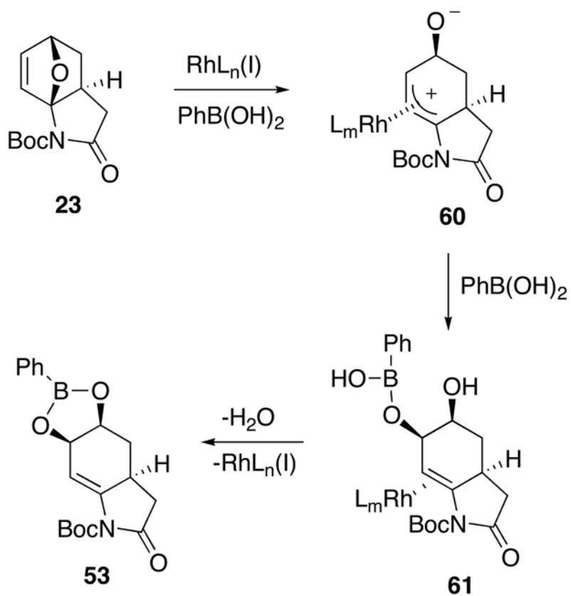
Scheme 11. Rh(I) Catalyzed Reaction using \text{PhB}(\text{OH})_2
