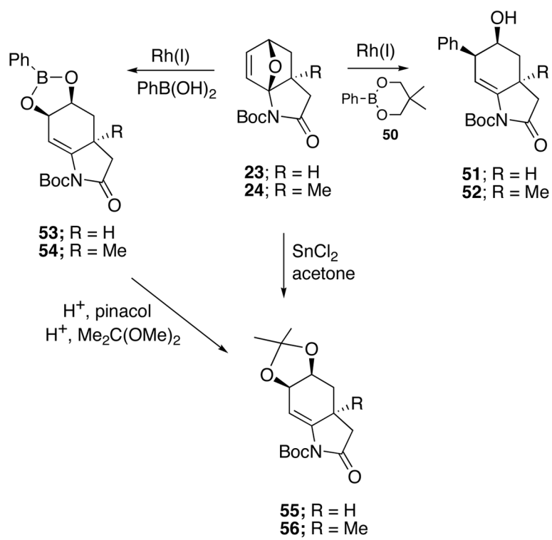
Scheme 9. Rh(I)-Catalyzed Addition of Arylboronic Acids to the IMDAF Cycloadducts
