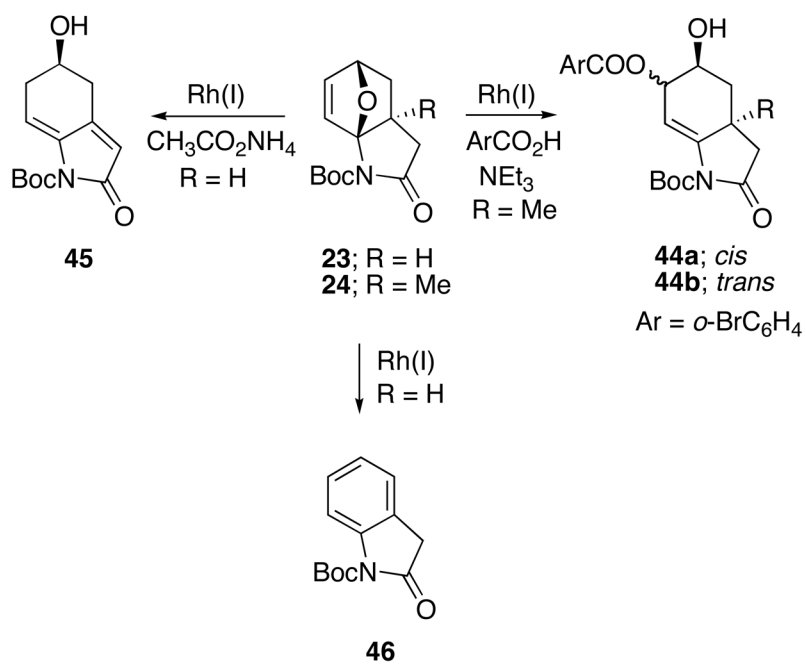
Scheme 7. Rh(I)-Catalyzed Ring Opening Reactions Using Carboxylates as the Nucleophile
