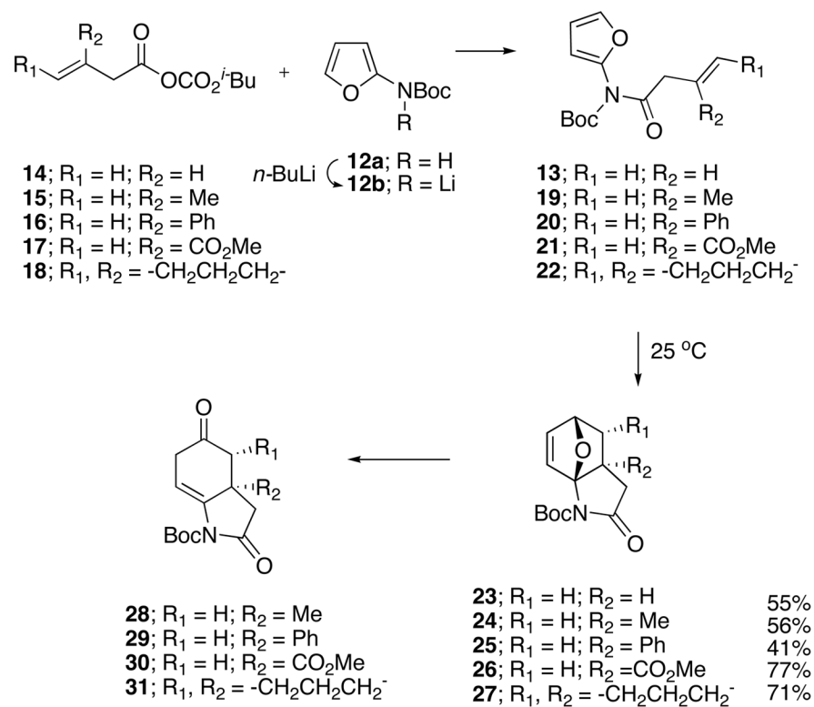
Scheme 4. IMDAF Cycloaddition of the 2-Imidofuran System
