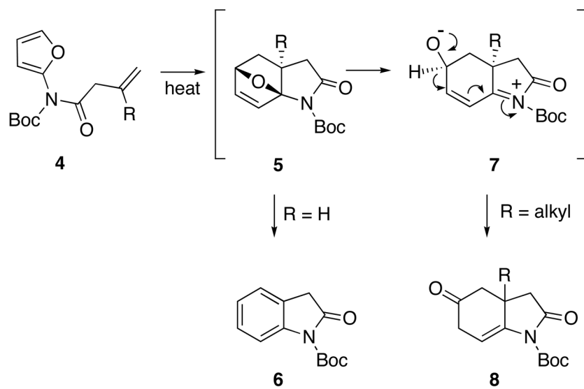
Scheme 2. IMDAF Reaction of Furanyl Carbamates
