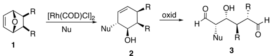
Scheme 1. Lautens' Oxabicyclic Ring Opening Protocol
