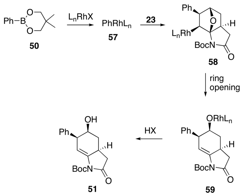
Scheme 10. Rh(I)-Catalyzed Reaction of the Oxabicyclic System Using 5,5-Dimethyl-2-phenyl-[1,3,2]-dioxaborinane (50)
