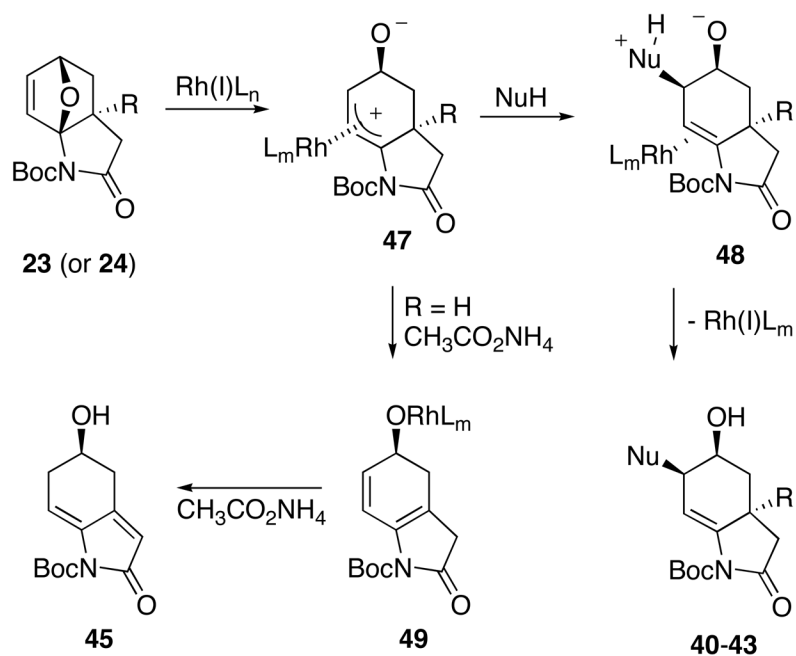
Scheme 8. Proposed Mechanism for the Rh(I)-Catalyzed Ring-Opening Reactions
