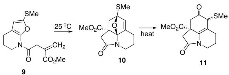
Scheme 3. Isolation of the Aza-oxabicyclic Cycloadduct
