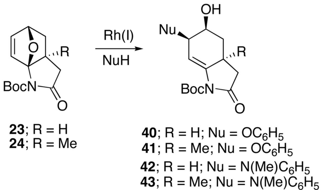
Scheme 6. Rh(I) Catalyzed Ring Opening of the 10-Oxa-2-azatricyclodecene System
