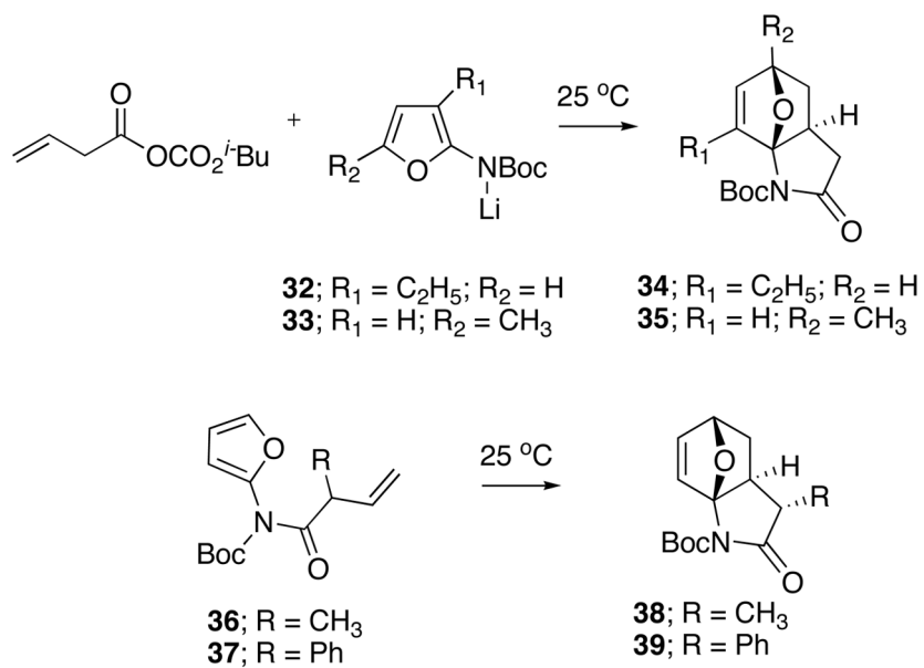
Scheme 5. More Heavily Substituted Systems
