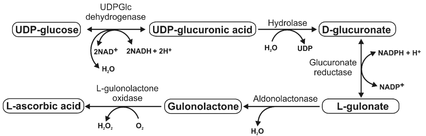
Figure 1. Ascorbate Metabolism
