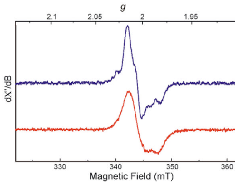
Figure 1. EPR spectra of the diiron(III,IV)-W* intermediate generated in the reaction of reduced ToMOH-I100W with O 2 . The reaction was quenched at 4 s using natural-abundant diiron(II) protein (blue) or at 3.5 s using 57 Fe-enriched protein (red).
