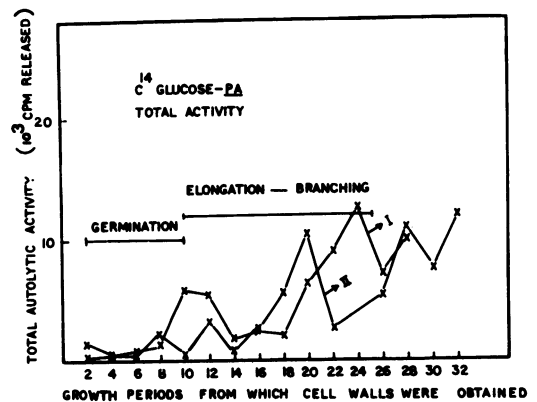
FIG. 3. Total autolytic activity associated with cell walls from various growth periods of wild type (PA) from two experiments (I and II). Cell walls were labeled with ^{14} C-glucose.
