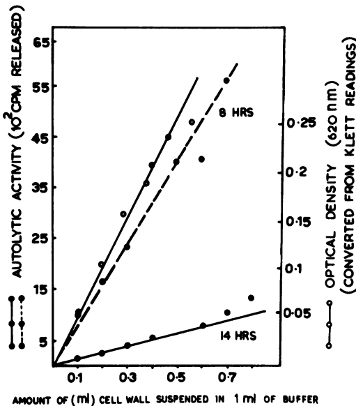
FIG. 1. Linear relationships of amount of homogenized cell wall suspension to its optical density and autolytic capacity. Autolytic capacity was determined for cell walls at 8 and 14 hr of growth.
