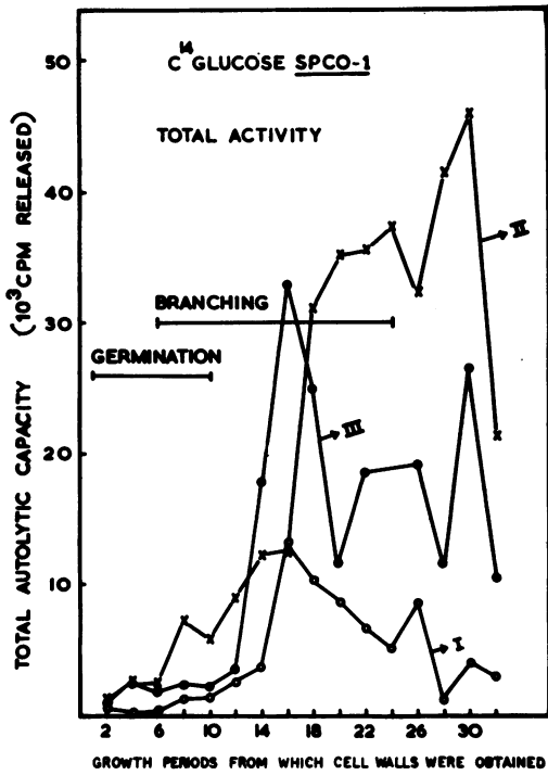
FIG. 4. Total autolytic activity associated with cell walls from various growth periods of spco-1 from three experiments (I, II, III). Cell walls were labeled with ^{14}\text{C} -glucose.
