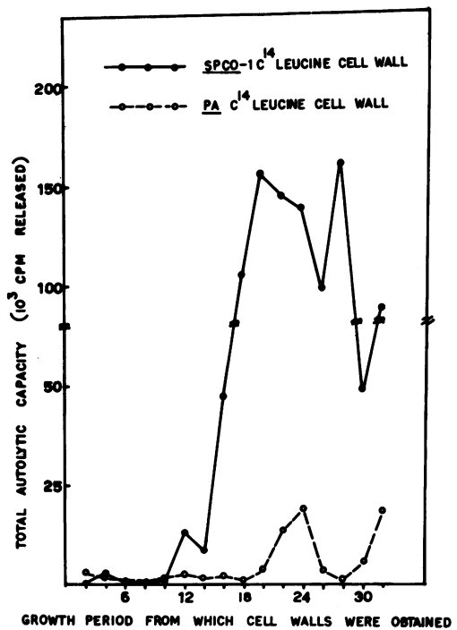
FIG. 5. Total autolytic activity associated with ^{14}\text{C} -leucine labeled cell walls from various growth periods of PA and spco-1 .
