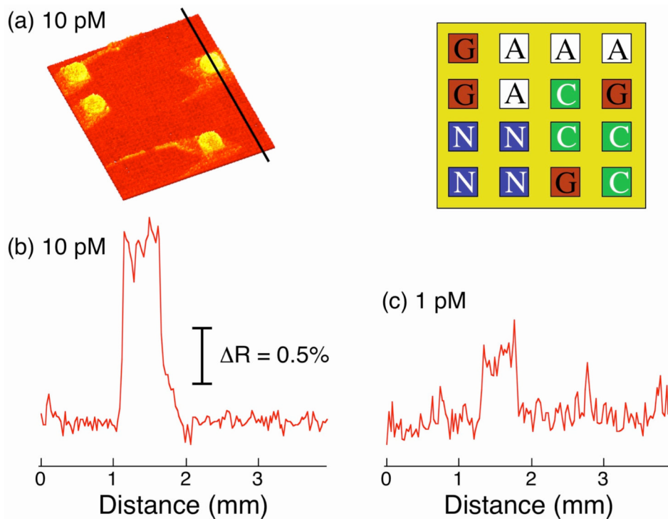
Figure 2. Detection and identification of single base pairs and mismatches in short synthetic DNA sequences. A four-component DNA microarray consisting of DNA probes ( P A , P C , P G and P N ) was used. The ligation reaction was first performed in the presence of 10 pM target DNA ( T ) for 2 h at room temperature. The surface was then denatured with 8 M urea and rinsed with hybridization buffer. (a) An SPR difference image was obtained by subtracting images taken before and after the exposure of the ligated array to L C -modified gold nanoparticles. SPR signal increase due to hybridization adsorption of the nanoparticles was observed only at the P G array elements, where the probe sequence is perfectly matched to T . Non-specific adsorption was not observed either on the other probe array elements or on the PEG background. (b) A line profile taken from the SPR difference image in (a) for 10 pM target DNA. (c) A line profile taken from an SPR difference image obtained from a separate experiment using 1 pM T . The percent reflectivity scale is the same for both (b) and (c). The ligation reaction with 1 pM DNA was performed at a temperature of 45 °C.
