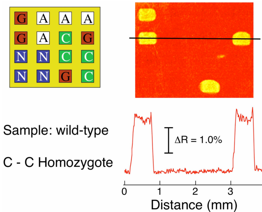
Figure 3. SNP genotyping of a 1 nM PCR amplicon of wild-type genomic DNA. A four-component probe DNA microarray ( P_A , P_C , P_G and P_N ) was first exposed to a solution containing target PCR amplicon, ligation probe DNA and Taq DNA ligase for 2 h followed by a surface denaturation step. The SPR difference image after specific hybridization adsorption of L^C -modified nanoparticles onto the ligated microarray is shown along with the corresponding array pattern and line profile. An SPRi signal increase observed at only the P_G array elements identifies the wild-type sample as being a C-C homozygote.
