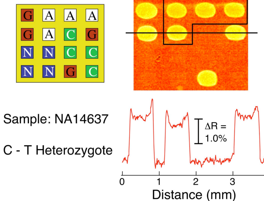
Figure 5. SNP genotyping of a 1 nM PCR amplicon of genomic DNA sample NA14637. An SPR difference image was obtained by subtracting images taken before and after the exposure of \text{L}^{\text{C}} -modified nanoparticles to a ligated microarray prepared in an identical manner to that in Figures 3 and 4. The array pattern and corresponding line profile are also shown. The SPRI signal increase observed at both the \text{P}_{\text{G}} and \text{P}_{\text{A}} (boxed) elements identifies the NA14637 sample as a C-T heterozygote.
