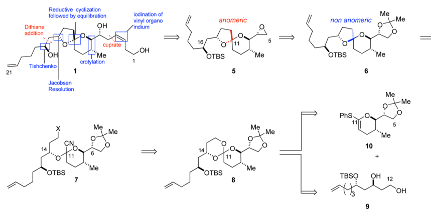
Figure 2. Disconnection plan
