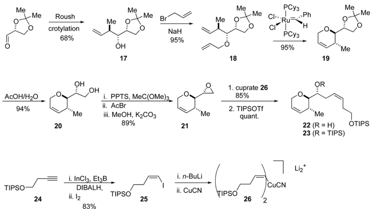
Scheme 3. Synthesis of DHP and Organocuprate
