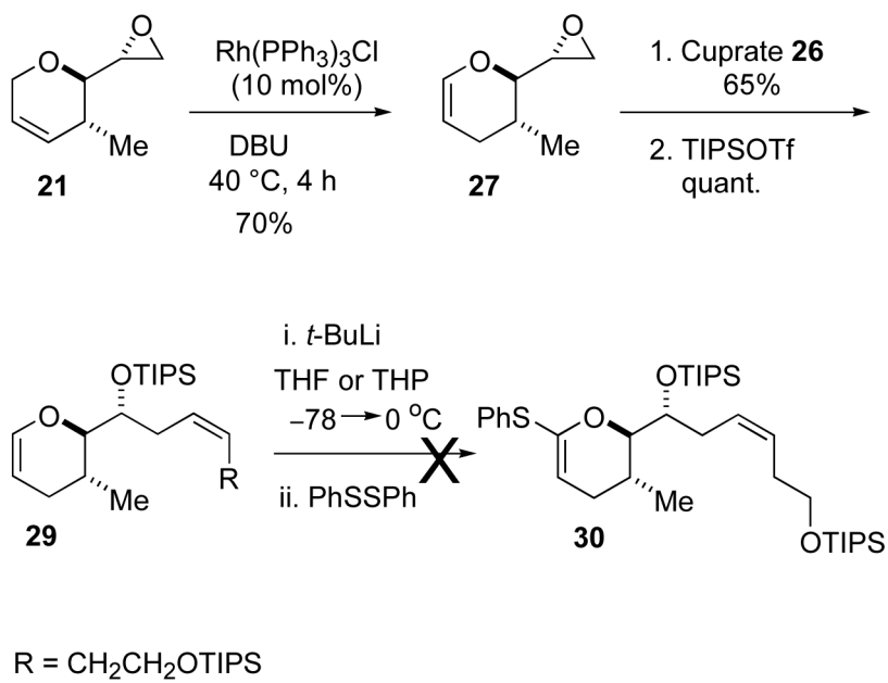
Scheme 4. Attempted lithiation
