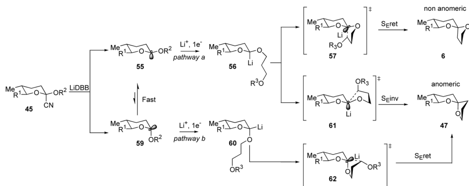
Scheme 12. Mechanism of Cyclization
