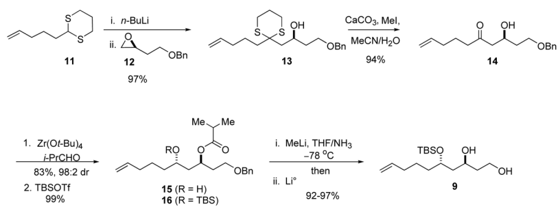
Scheme 2. Synthesis of diol
