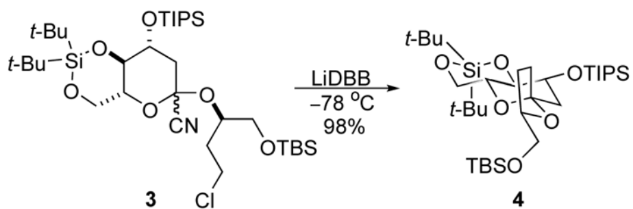
Scheme 1. Stereoselective preparation of non-anomeric spiroacetal
