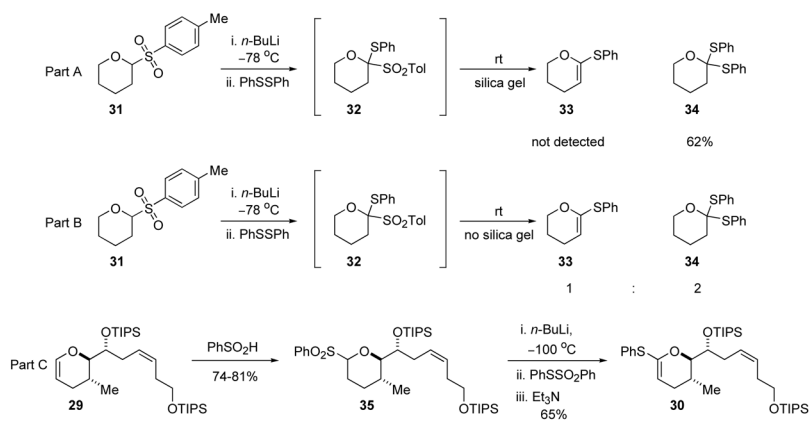
Scheme 5. Sulfone mediated thioketene acetal synthesis
