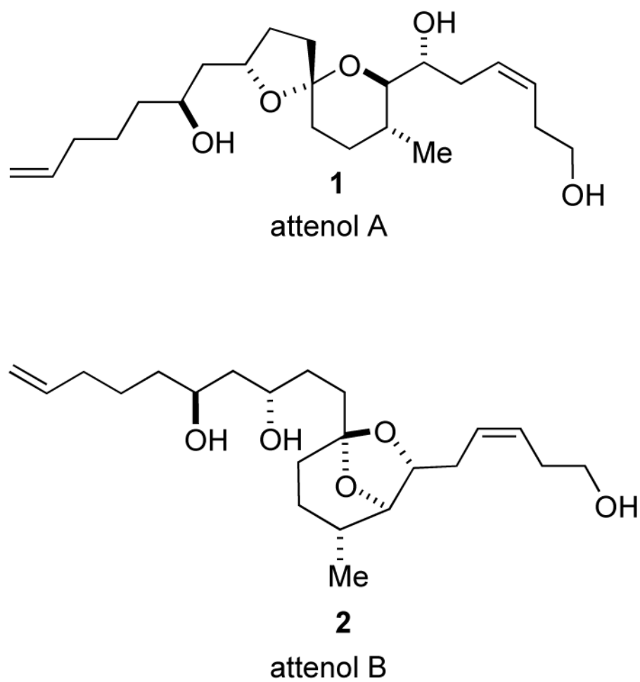
Figure 1. Attenol A and B
