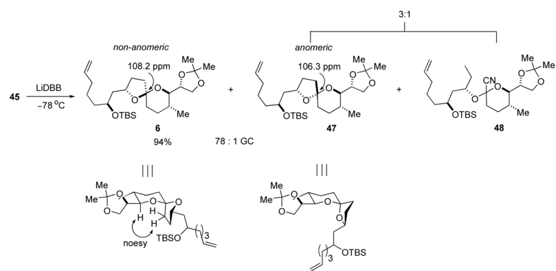
Scheme 10. Reductive cyclization
