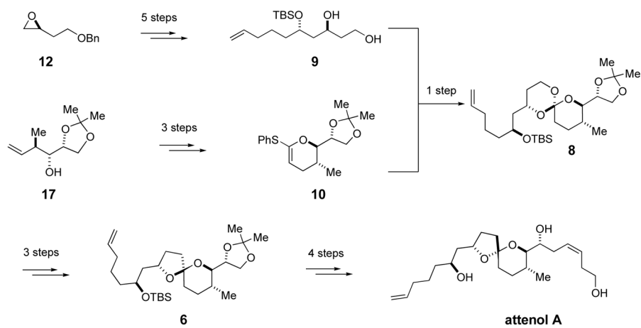
Scheme 13. Summary of the Synthesis
