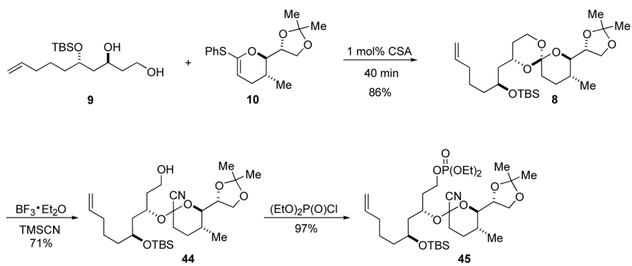
Scheme 9. Spiro orthoester and cyclization precursor synthesis
