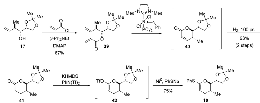
Scheme 8. Revised strategy to thioketene acetal
