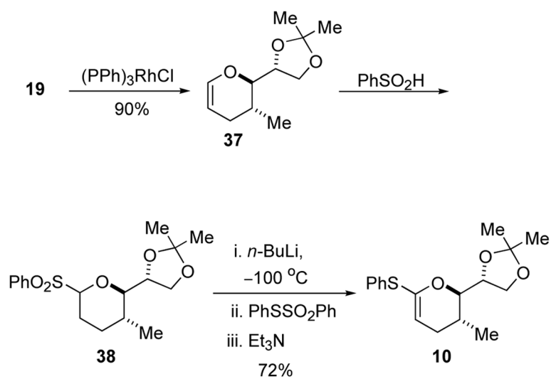
Scheme 7. Truncated thioketene acetal
