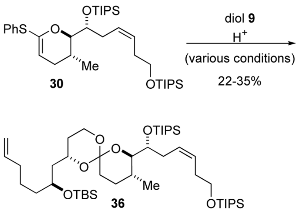
Scheme 6. Disappointing orthoester synthesis
