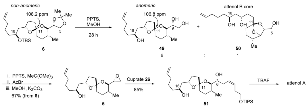
Scheme 11. Completion of the synthetic sequence
