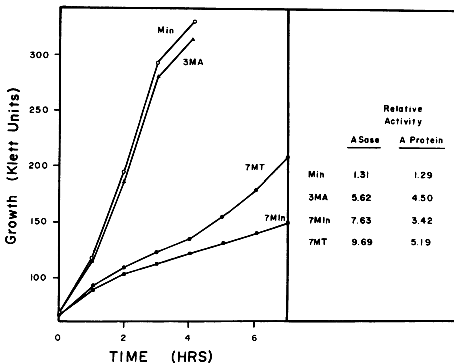
FIG. 4. Derepression and growth inhibition by 3-methylanthranilic acid (3MA), 7-methylindole (7MIn), and 7-methyltryptophan (7MT) in W1485 tna . Cultures were harvested at the end of the growth period and cell-free extracts were prepared. Enzyme activities are relative to the level of enzymes in W1485 tna grown in minimal medium.
