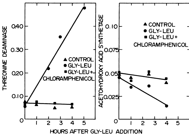
FIG. 3. Effect of glycyL-leucine on threonine deaminase and acetohydroxy acid synthetase levels. Glycyl-leucine (1 mM) was added to log-phase cultures of E. coli K-12. Samples were removed at 1-hr intervals, and threonine deaminase and acetohydroxy acid synthetase levels were measured. Enzyme activities are expressed in micromoles per minute per milligram of protein. The level of chloramphenicol was 200 \mu\text{g/ml} .
