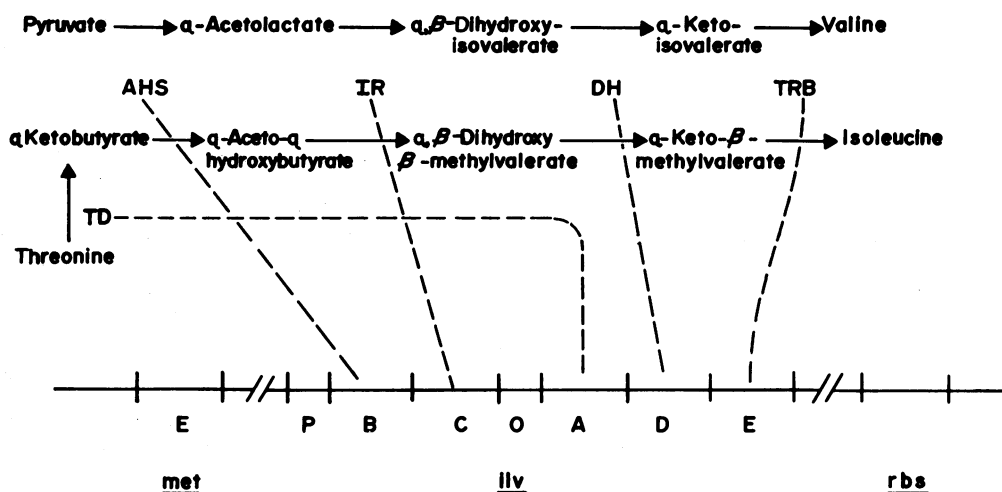
FIG. 1. Enzymatic steps in isoleucine and valine biosynthesis and the corresponding structural genes. In addition to the structural genes, two controlling elements, ilvO and ilvP , are represented. Modified from Ramakrishnan and Adelberg (6).
