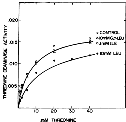
FIG. 5. Effects of glyceryl-leucine, leucine, and isoleucine on the activity of threonine deaminase in extracts of strain CU45. All assays were performed at pH 7. Enzyme activity is expressed in micromoles per minute per milligram of protein.
