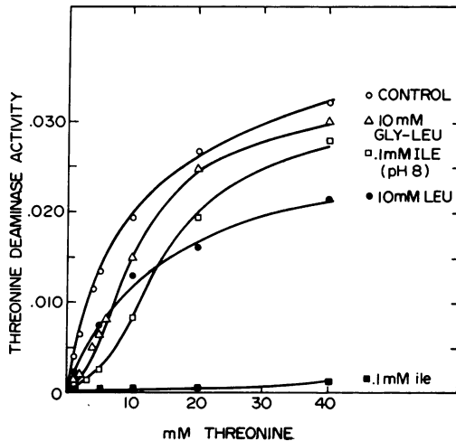
FIG. 4. Effects of glyceryl-leucine, leucine, and isoleucine on the activity of threonine deaminase in extracts of strain K-12. Control assays and assays in the presence of glyceryl-leucine and leucine were performed at pH 7. At pH 8, the inhibition by leucine was the same as at pH 7. The assay in the presence of isoleucine was performed at pH 8. Assays performed at pH 7 in the presence of 0.1 mM isoleucine resulted in complete inhibition of threonine deaminase at all but the highest threonine concentrations. Enzyme activity is expressed in micromoles per minute per milligram of protein.
