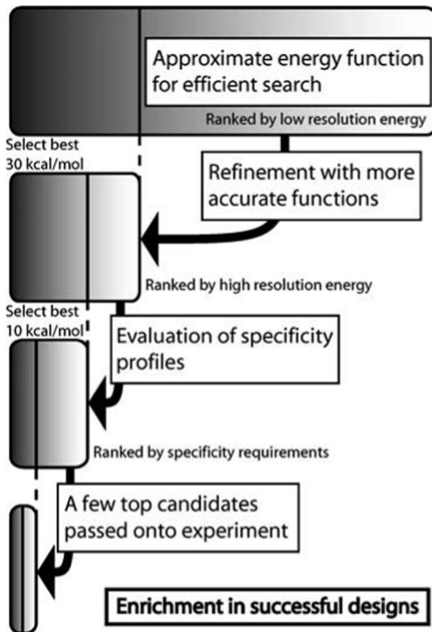
Figure 2. Hierarchical design protocol
