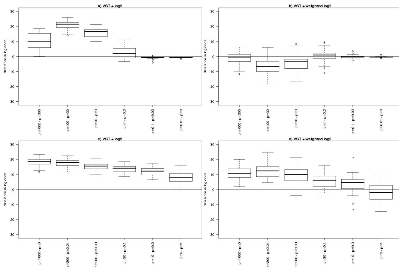
Figure 2 Comparison of spike log-odds obtained for a particular contrast in the linear model fitted to the entire spike-in experiment of 48 arrays. On the left we show the difference between the log-odds obtained after VST and the log-odds obtained after a \log_2 transformation. On the right, we show the difference between VST and a linear model incorporating \log_2 variances as weights (see [7]). In the top panels, we show six independent contrasts with the closest spike concentrations. The bottom panel shows six independent contrasts from the same linear model, but chosen to provide a range in anticipated log-ratios (the finer differences being to the right of the panel). In all cases, a positive value indicates greater log-odds obtained (i.e. more evidence for differential expression) after VST.
