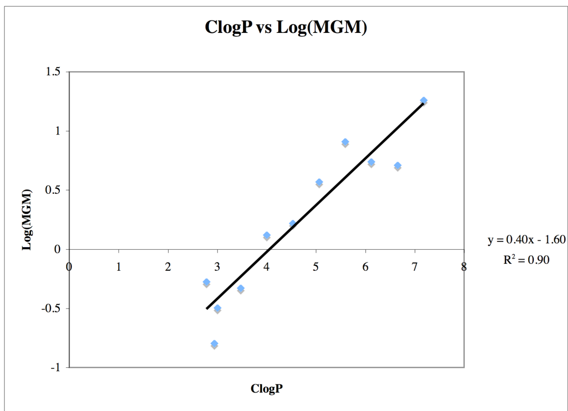
Figure 3. ClogP vs. Log(MGM).
