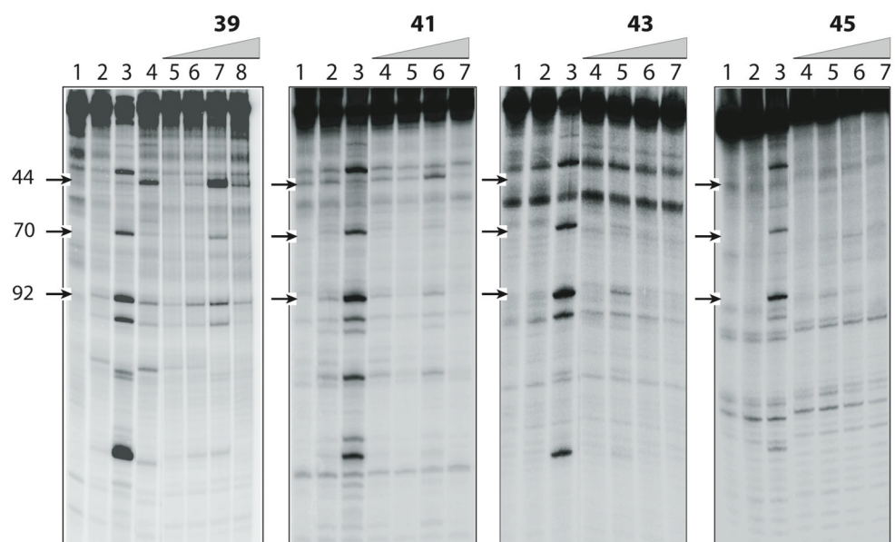
Figure 2. Lane 1: DNA alone; lane 2: top1 alone; lane 3: + CPT (1 \mu M); in the first panel, lane 4: top1 + NSC 314622 (100 \mu M); lanes 5–8 (for compound 39 ) and lanes 4–7 (for compounds 41 , 43 , and 45 ): top1 + indicated compound at 0.1, 1, 10, and 100 \mu M, respectively. Number on left and arrows indicate cleavage site positions.
