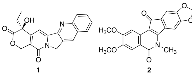
Figure 1. Representative topoisomerase I inhibitors.
