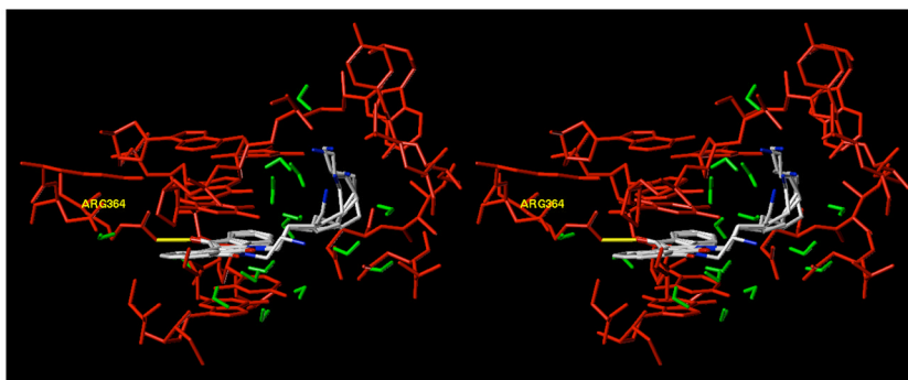
Figure 4. Overlay of the hypothetical models derived from PDB code 1K4T for compounds 37 , 39 , 41 , 43 , 45 , and 47 (colored by atom type) in ternary complex with DNA (red) and top1 (red). Water molecules are indicated in green and the hydrogen bond between the analogues and Arg364 is shown in yellow. The figure is programmed for wall-eyed (relaxed) viewing.
