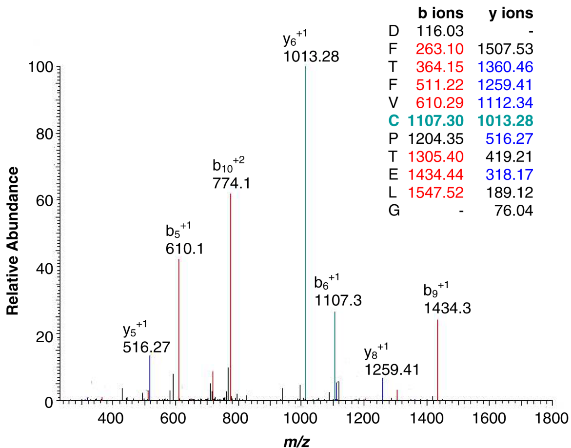
Figure 4. Nano-LC-MS/MS spectrum of the DCP-Bio1-labeled peptide of C165S AhpC containing an adduct at Cys46
