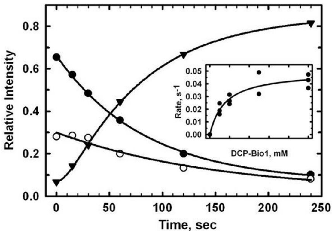
Figure 5. Kinetic Studies of Modification Rates of Sulfenic Acid-Containing Papain with DCP-Bio1 Papain in 25 mM potassium phosphate buffer, pH 7, with 1 mM EDTA was incubated with DCP-Bio1 and 2 equiv of hydrogen peroxide, with the time of reaction taken after addition of the oxidant. At each time point a 50 \mu L sample containing 5 nmol papain was applied to a Bio-Gel P6 spin column to remove small molecules and exchange the buffer into 10 mM ammonium bicarbonate, then the mass spectra were obtained after rapid addition of acetonitrile and formic acid and injection into an Agilent LC/MSD TOF MS. Data plotted from one reaction with 5 mM DCP-Bio1 show the loss of the thiol form of papain (closed circles), the appearance of the covalent adduct with DCP-Bio1 (inverted triangles), and the putative sulfenic acid form (open circles) over time. Data from multiple concentrations of reagent and three independent experiments were fit to a A \rightarrow B \rightarrow C kinetic model as described in the text, giving a single first order rate in this experiment of 0.024 \pm 0.007 \text{ s}^{-1} for formation of the sulfenic acid form of papain, and a second, saturable step with a maximal rate of 0.050 \pm 0.005 \text{ s}^{-1} and apparent K_m = 0.77 \pm 0.24 \text{ mM} for reaction of DCP-Bio1 with the sulfenic acid of papain.
