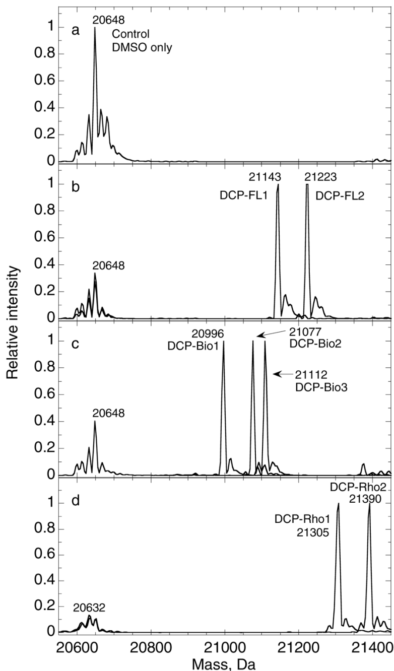
Figure 3. Electrospray ionization mass spectrometry analysis of adducts with the sulfenic acid form of C165S AhpC
