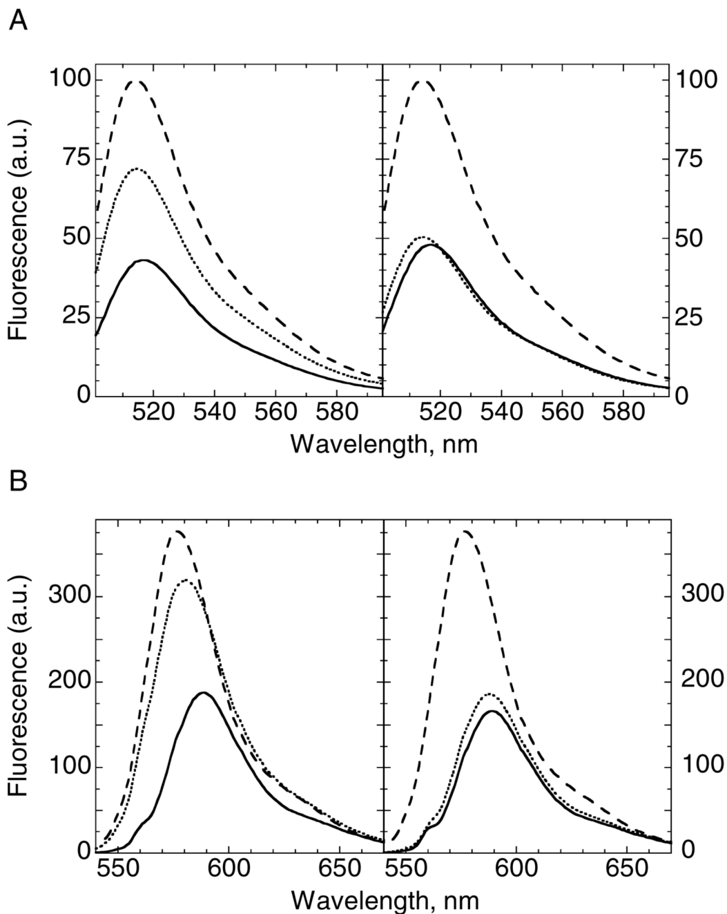
Figure 1. Fluorescence spectra of fluorescein- (A) and rhodamine-linked (B) reagents before (dotted) and after (solid) reaction with cysteine sulfenic acid-containing AhpC
