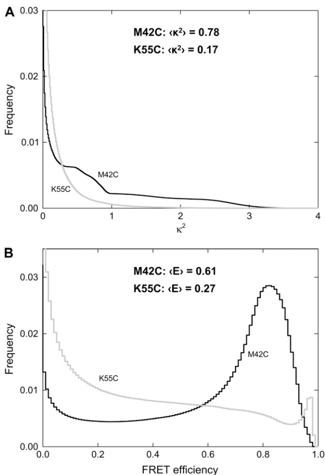
FIGURE 8 Results from ensemble averaging of the data as described in the text. The frequency at which each value of (A) the orientation factor and (B) the given FRET efficiency arise are indicated with the fluorophores attached to site 42 (solid lines) and site 55 (shaded lines).
