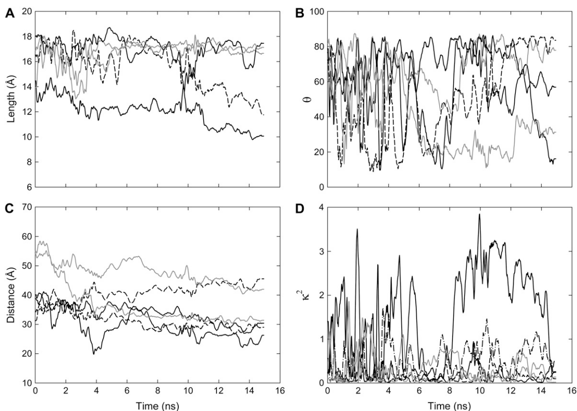
FIGURE 4 Properties of the fluorophores when attached to residue 55 in the periplasmic domain of MscL. All symbols are as for Fig. 3. The relatively common low \kappa^2 values arise from the AlexaFluor headgroups lying perpendicular to one another.
