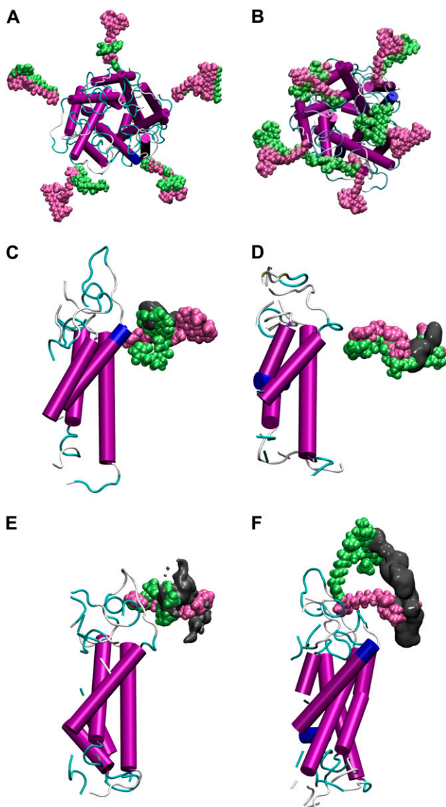
FIGURE 5 Locations of the fluorophores at the beginning ( pink ) and end ( green ) of each simulation. Results are shown for 15-ns simulations when the fluorophores are attached to (A) residue 42 and (B) residue 55. Similar results are shown for simulations of a single fluorophore and only part of the protein: (C) AF488 attached at residue 42 (50-ns simulation); (D) AF568 attached to residue 42 (50-ns simulation); (E) AF488 attached to residue 55 (30-ns simulation); and (F) AF568 attached to residue 55 (30-ns simulation). The volume of space sampled by the central oxygen in the fluorophore headgroup is indicated by the gray surface in the later pictures.
