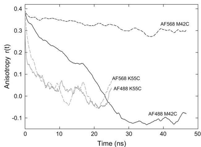
FIGURE 6 Fluorescence anisotropy decay curves calculated from simulations of a single fluorophore attached to MscL. Results are shown for AF488 (solid line) and AF568 (dashed line) attached to site 42 (solid color) and site 55 (shaded line).
