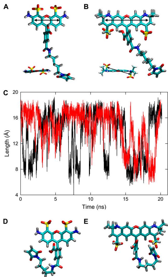
FIGURE 2 Structures of AlexaFluor dyes. The geometry-optimized structures found in ab initio calculations are shown for (A) AF488 and (B) AF568. The direction of the transition moment is indicated by the arrow. (C) The length of the dyes, measured from the central oxygen in the headgroup to the furthest carbon in the linker is plotted during simulations in which AF488 (black) or AF568 (red) is immersed in water. Compact structures sampled during the molecular dynamics simulations are shown for (D) AF488 and (E) AF568.
