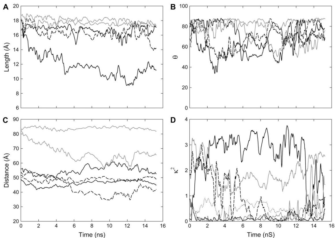
FIGURE 3 Properties of the fluorophores when attached to residue 42 near the lipid-water interface on MscL. Running average values of the length of the fluorophores (A), and angle between the transition moment and membrane normal (B) are shown during the simulations for each fluorophore, where results for the three AF488 molecules are shown as solid or dashed curves and two AF568s in shading. The running average distance between each of the AF488 and AF568 fluorophore pairs (C) and the orientation factor for transfer between them (D) are shown where the nearest neighbor pairs are shown as solid or dashed lines, and next nearest-neighbor pairs are shown in shading.
