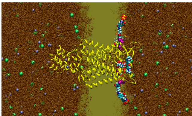
FIGURE 1 Simulation system. AlexaFluor488 and AlexaFluor568 (shown in space-filling representation) are attached to residue 42 of the MscL protein (yellow) embedded in a lipid bilayer (light brown), surrounded by water (brown), sodium (purple), and chloride (green) ions. The front half of the lipid, water, and ion atoms have been removed to reveal the protein and dye molecules.
