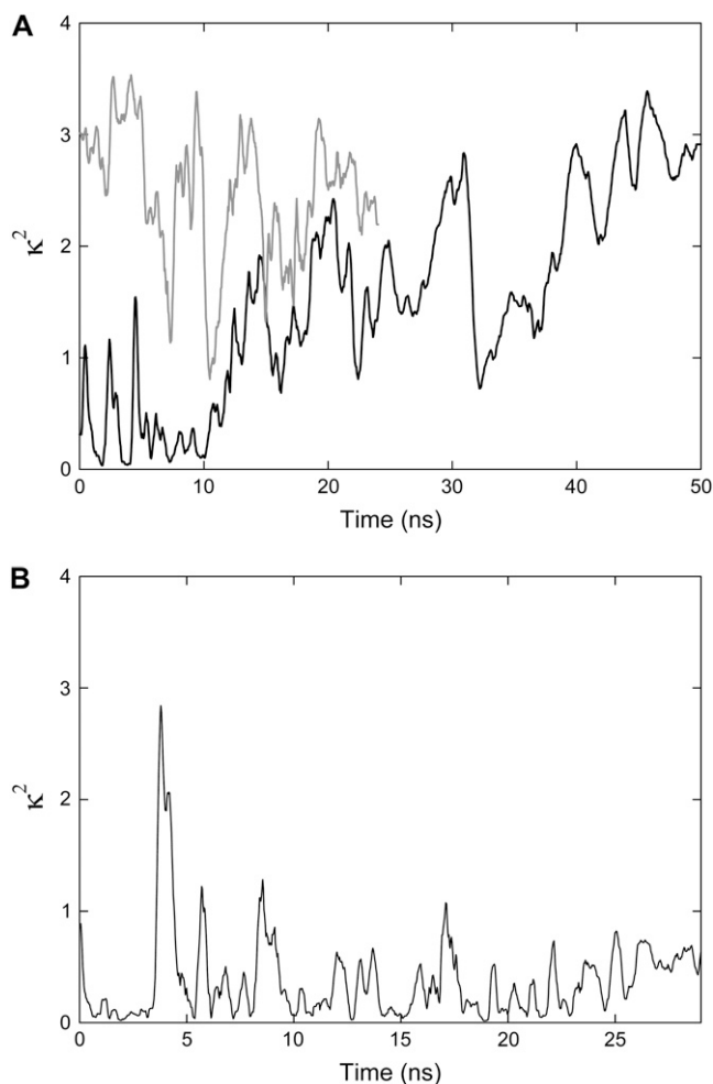
FIGURE 7 Running average orientation factor calculated from simulations of just one fluorophore and part of the protein. Results are calculated with fluorophores attached to (A) site 42 and (B) site 55. Results of a second independent simulation for site 42 are also indicated by the shaded line.
