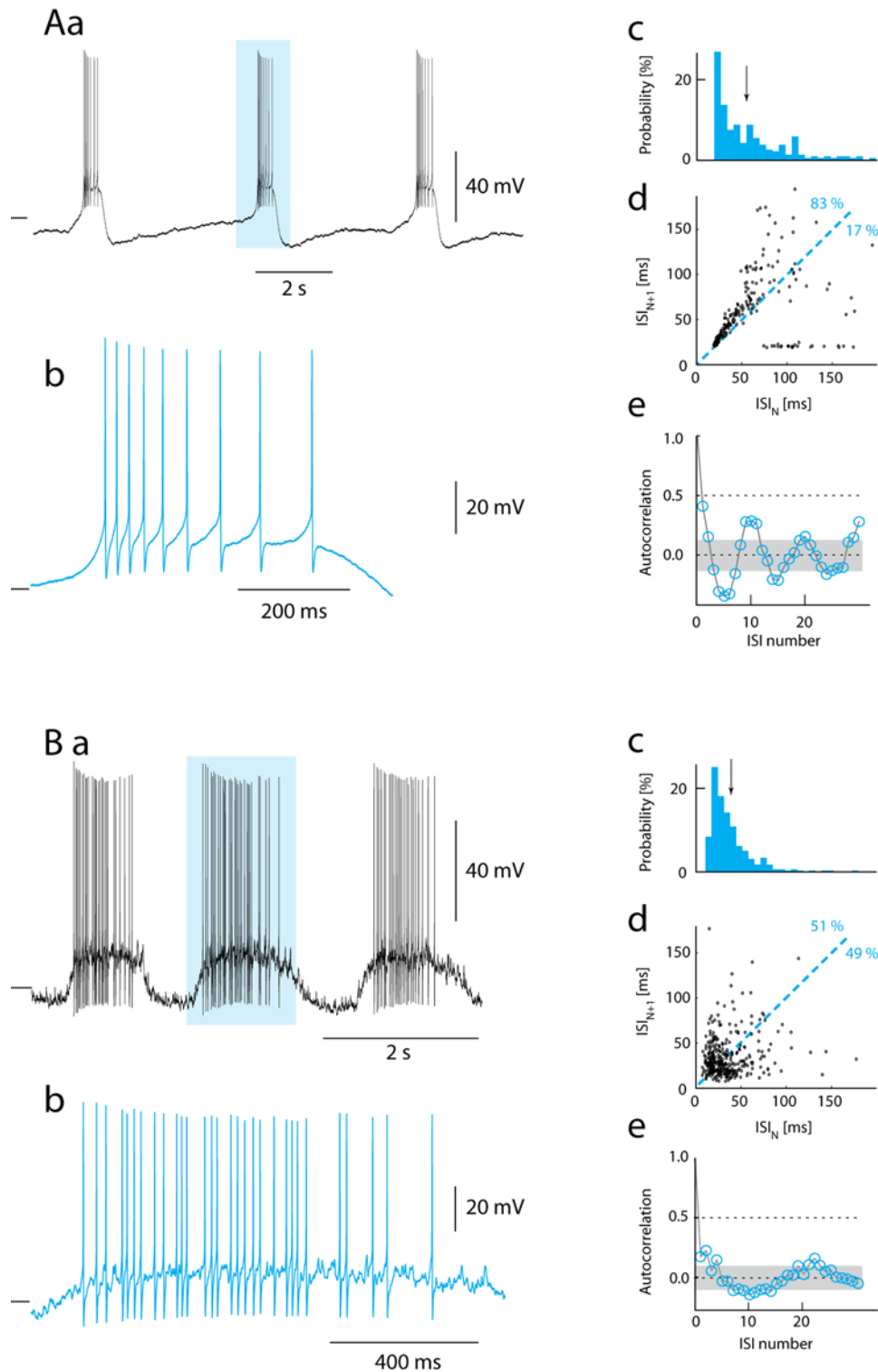
Figure 6. Presence and absence of spike frequency adaptation (SFA) during bursting. (Aa) SFA in intracellular recording from motoneuron in slice during NMDA induced bursting. (Ab) Single burst highlighted in (Aa) show gradual increase in ISI. (Ac) Histogram of ISI. The mean ISI is 55 ms (arrow). (Ad) Plot of ISI_N against ISI_{N+1} shows significantly greater proportion of points above than below the ISI_N = ISI_{N+1} line (83.2% above, total N = 239 ), which is evidence of spike frequency adaptation. In addition, ISIs are correlated with their neighbors (correlation coefficient = 0.41), as expected when ISI are influenced by AHP conductance and the burst pattern is reproduced after 10 spikes (Ae). Gray area represents the 5% confidence limit \pm 1.96/\sqrt{N} . (Ba) Recording from a MN in a functional spinal network during rhythmic motor activity. (Bb) A highlighted cycle from (Ba) shows irregular spike times and no SFA. (Bc) Histogram of ISI. The mean ISI is 34 ms (arrow) (Bd) A plot of ISI_N against ISI_{N+1} illustrates no discrepancy of points above and below the ISI_N = ISI_{N+1} line (51.3% above, total N = 362 ), which demonstrates absence of SFA. Furthermore, there is only a marginal correlation of ISI with neighbors (correlation coefficient = 0.18), as expected with negligible AHP conductance (Be). Gray area represents the 5% confidence limit \pm 1.96/\sqrt{N} . Tick marks to the left represent -80 mV (A) and -60 mV (B). Inter-burst-intervals are omitted in analysis. doi:10.1371/journal.pone.0003218.g006
