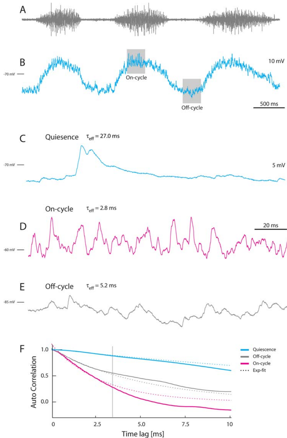
Figure 4. Temporal characteristics of sub-threshold V_m -fluctuation in motoneurons during quiescence and in the on- and off-cycle during scratching. (A) Hip-flexor nerve recording during scratch. (B) Concurrent V_m in MN, spikes avoided with -2.5 nA hyperpolarizing current. Shaded regions mark the selected area of on- and off-cycle illustration below. Sample trace of V_m in quiescence (C) (note time-course of spontaneous synaptic potentials) and in the on-cycle (D) and off-cycle (E). D and E are from the shaded boxes in B. (F) The auto-correlation sequence of each sample trace. Blue is from quiescent trace (C), gray is from the off-cycle trace (E), and red is the on-cycle trace (D). The effective time constant of each trace is obtained by fitting an exponential decay function (broken lines) to the initial 3 ms (until the vertical gray line). The time constants are \tau_{\text{eff}} = 2.8 ms (on-cycle activity), \tau_{\text{eff}} = 5.2 ms (off-cycle activity) and \tau_{\text{eff}} = 27.0 ms (quiescence). C–E are on the same time scale. doi:10.1371/journal.pone.0003218.g004
