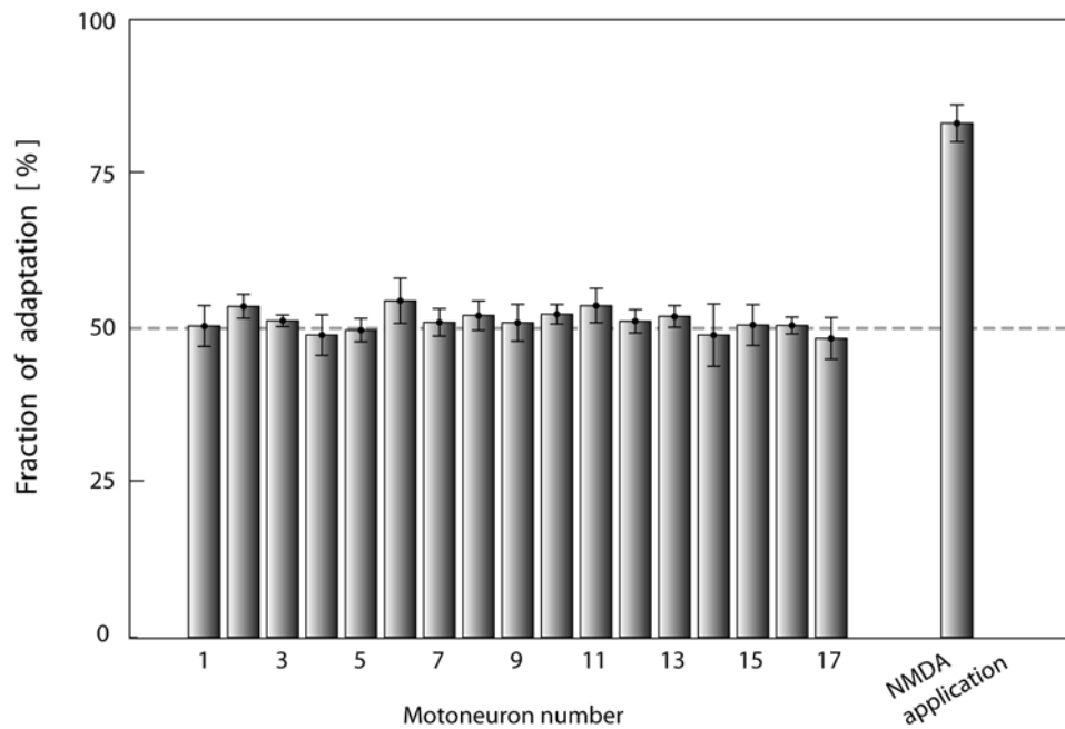
Figure 7. Spike frequency adaptation during NMDA induced bursts but absent during scratching. The number of points above the ISI_N = ISI_{N+1} -line in a ISI-return map (Figure 7Ad and 7Bd) divided by the total number of intervals ( \times 100\% ) for all MNs including the NMDA induced bursting data from slice experiment for comparison. The network induced bursting have little or no SFA since there is an even amount of points above as below. In contrast, the NMDA-activated bursting has a much larger fraction above the line reflecting the high degree of SFA. Error bars are SE = \frac{\sqrt{K \cdot 0.25}}{K} , where K total number of ISI. doi:10.1371/journal.pone.0003218.g007
