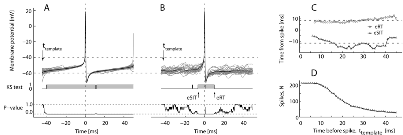
Figure 3. Effective recovery time and synaptic integration time during scratching. Peri-spike V_m distribution in quiescence (A) ( n = 50 ) and during scratching (B) ( n = 29 ). Top, superimposed data traces (gray) with mean V_m in black. Middle, KS-test. Bottom, P-values for the KS test. The effective synaptic integration time (eSIT) and effective recovery time (eRT), defined as the time periods before and after the spike, in which the V_m distribution is significantly different from a template distribution (arrows), i.e. gray areas in the KS-graphs in the middle. P-values of the test is plotted below. (C) Estimates of eSIT and eRT versus position of the template distribution relative to the spike from (B) (broken lines represent mean values eSIT = 12.1 ms, eRT = 8.7 ms). (D) The number of traces in template distribution decreases with window length (from same data as in (B) and (C)). doi:10.1371/journal.pone.0003218.g003
