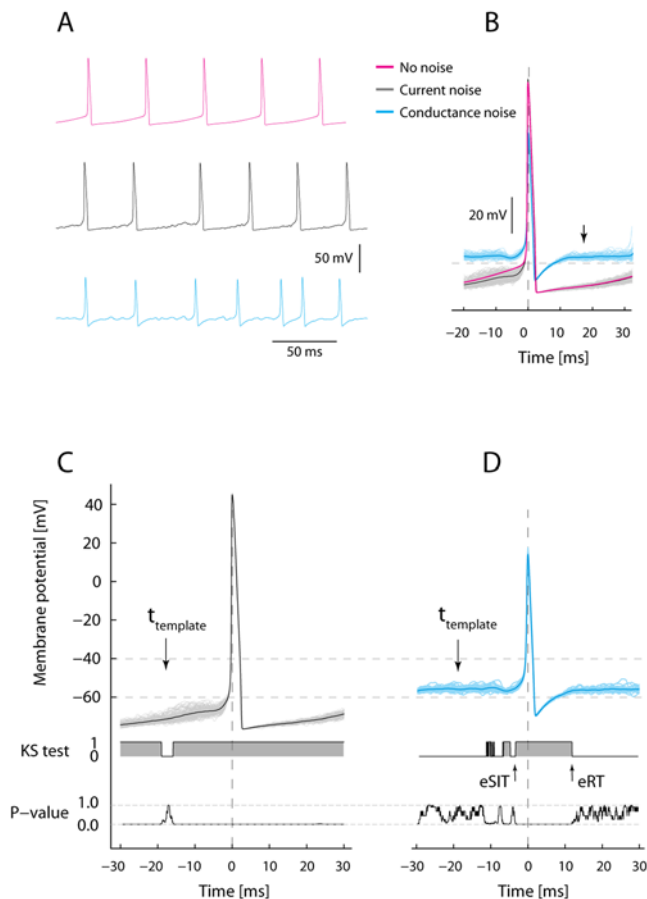
Figure 1. Computer simulation to illustrate firing pattern and AHP in current-based and conductance based models of synaptic input during repetitive firing. (A). Red top trace: Model with constant current injection, no other input. Black middle trace: Model with added current noise with same mean current as in top trace. Blue bottom trace: Model with same mean injected constant current and noise stemming from fluctuating conductance. (B). Spike triggered superimposed spikes. Red, black ( n=243 ) and blue ( n=72 ) traces are averages of spikes from (A). Notice the current-noise average closely overlap the no-noise trace (red) whereas the conductance-noise average (blue) rapidly reach pre-spike V_m -level (see arrow), because of increase in total conductance. (C) and (D) illustrate the statistical quantification of the evolution of V_m before and after the spike for traces in (B). A template distribution of V_m traces is chosen at an arbitrary time prior to the spike (see arrow at t_{\text{template}} ) for which the distribution at the rest of the time points is compared with. The outcome of comparison is shown as the KS-test trace below, 1 represents acceptance and 0 represents rejection of the hypothesis that they are different. Below is shown the P-values for the KS test. The distribution of V_m in (C) is different everywhere, whereas the distribution in (D) is only different up to and immediately after the spike. The time it takes to regain the pre-spike distribution following the spike is referred to as effective recovery time (eRT, arrow), while the endmost time of same distribution before the spike is referred to as effective synaptic integration time (eSIT, arrow). doi:10.1371/journal.pone.0003218.g001
