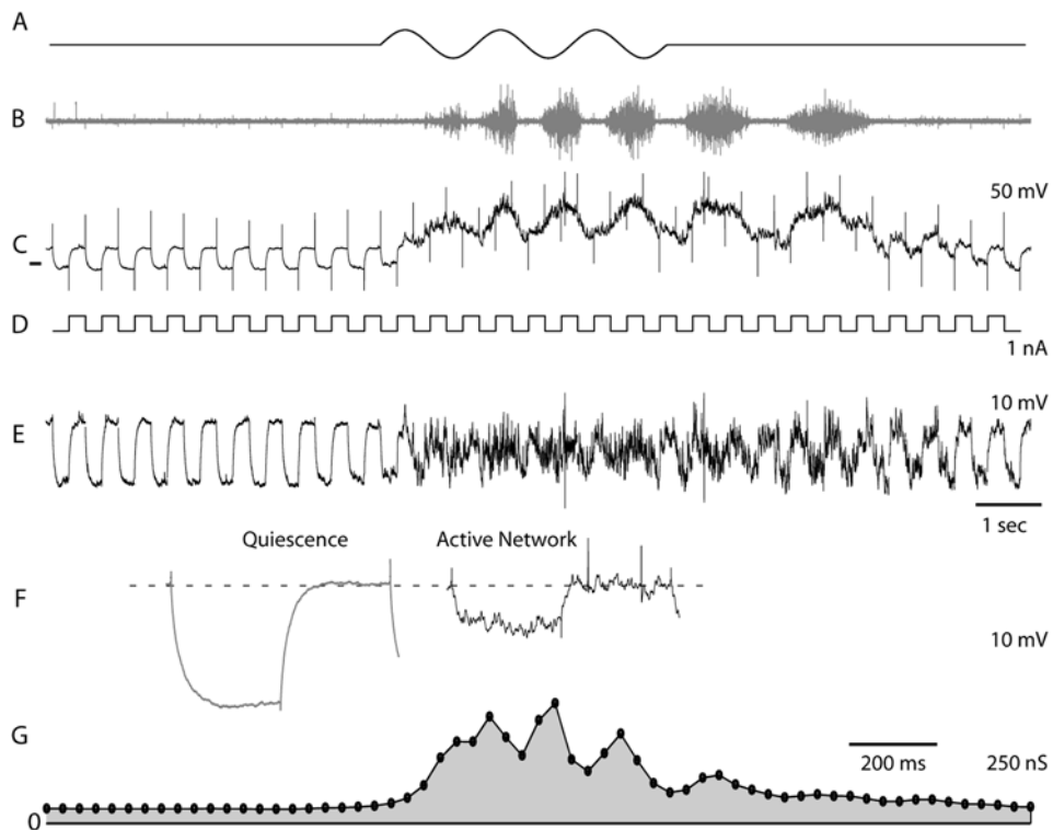
Figure 2. Increase in synaptic conductance during a single scratch epoch. (A) Cutaneous stimulation via sinusoidal movements of a glass rod on the hind-limb pocket skin. (B) Electro-neurogram from hip flexor nerve. (C) V_m from intracellular recording. Tick mark indicates V_m of -100 mV. (D) Current pulses of -0.7 nA from constant current level of -1.0 nA. (E) High-pass filtered V_m from (C) (cut off is 2 Hz). Transient artifacts removed. (F) left, average voltage deflections from (E) during quiescence ( n = 14 ), right during network activity ( n = 14 ). The average increase in conductance is 340%. Notice the occurrence of two spikes. (G) The membrane conductance as a function of time. The peak conductance during network activity is >800\% of the conductance during quiescence. doi:10.1371/journal.pone.0003218.g002
