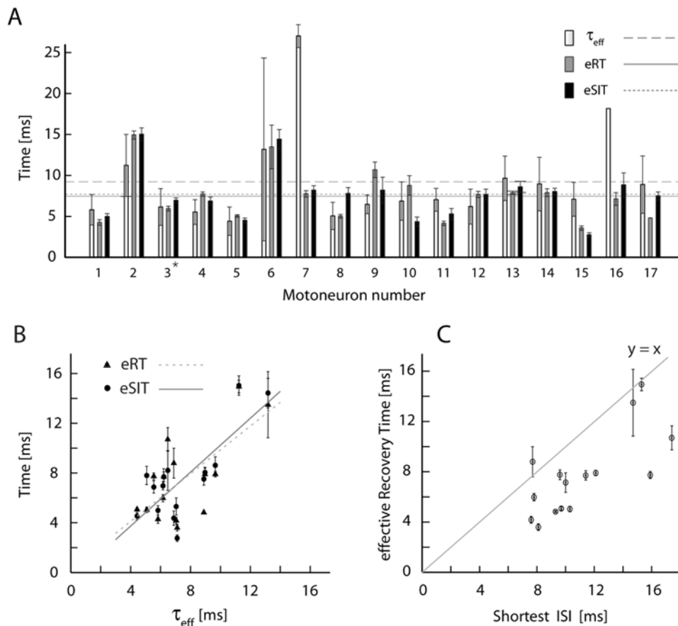
Figure 5. Time constants across the population of MNs. (A) The average \tau_{\text{eff}} (for ON-cycle), eRT and eSIT (mean \pm SE) as triplets bars for each cell. Horizontal lines represent population averages, \mu = 9.5 ms for \tau_{\text{eff}} , \mu = 7.5 ms for eRT, and \mu = 7.7 ms for eSIT. Cell 3 is marked with a \star and the sample cell used in figures 3, 4, 5. (B) eRT and eSIT plotted against \tau_{\text{eff}} show significant correlation. The lines are linear least square fits. (C) The shortest ISI at zero current injection plotted against the average eRT for each MN. Gray line is where x = y . doi:10.1371/journal.pone.0003218.g005
