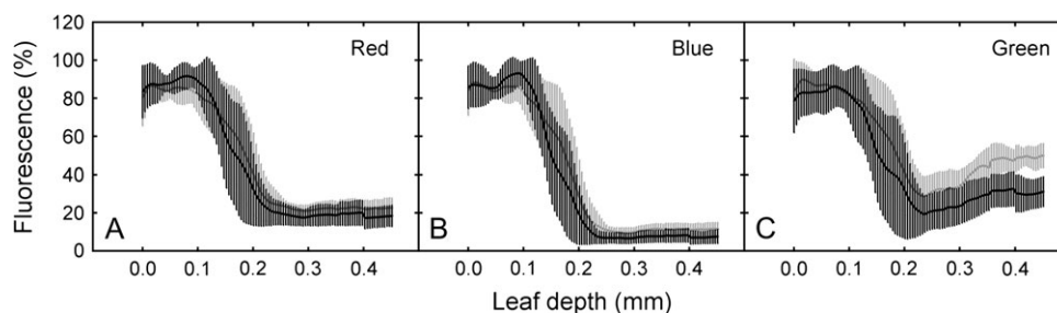
Fig. 4. Percentage chlorophyll fluorescence versus leaf depth for abaxial anthocyanic (black lines) and acyanic (grey lines) tissues of Begonia heracleifolia under red, blue, and green light. Error bars represent 95% confidence intervals for six replicates.
