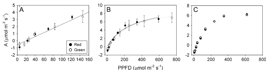
Fig. 5. Photosynthetic light response curves of abaxial acyanic/green (open circles, dotted lines) and anthocyanic/red (closed circles, solid lines) leaf tissues under red light. (A) Linear portion of the light response curves shown in (B); (B) light response curves from five leaves (with each having a single red and green section tested), and (C), a representative pair of light response curves derived from the same leaf. Error bars represent SE; n=5 .
