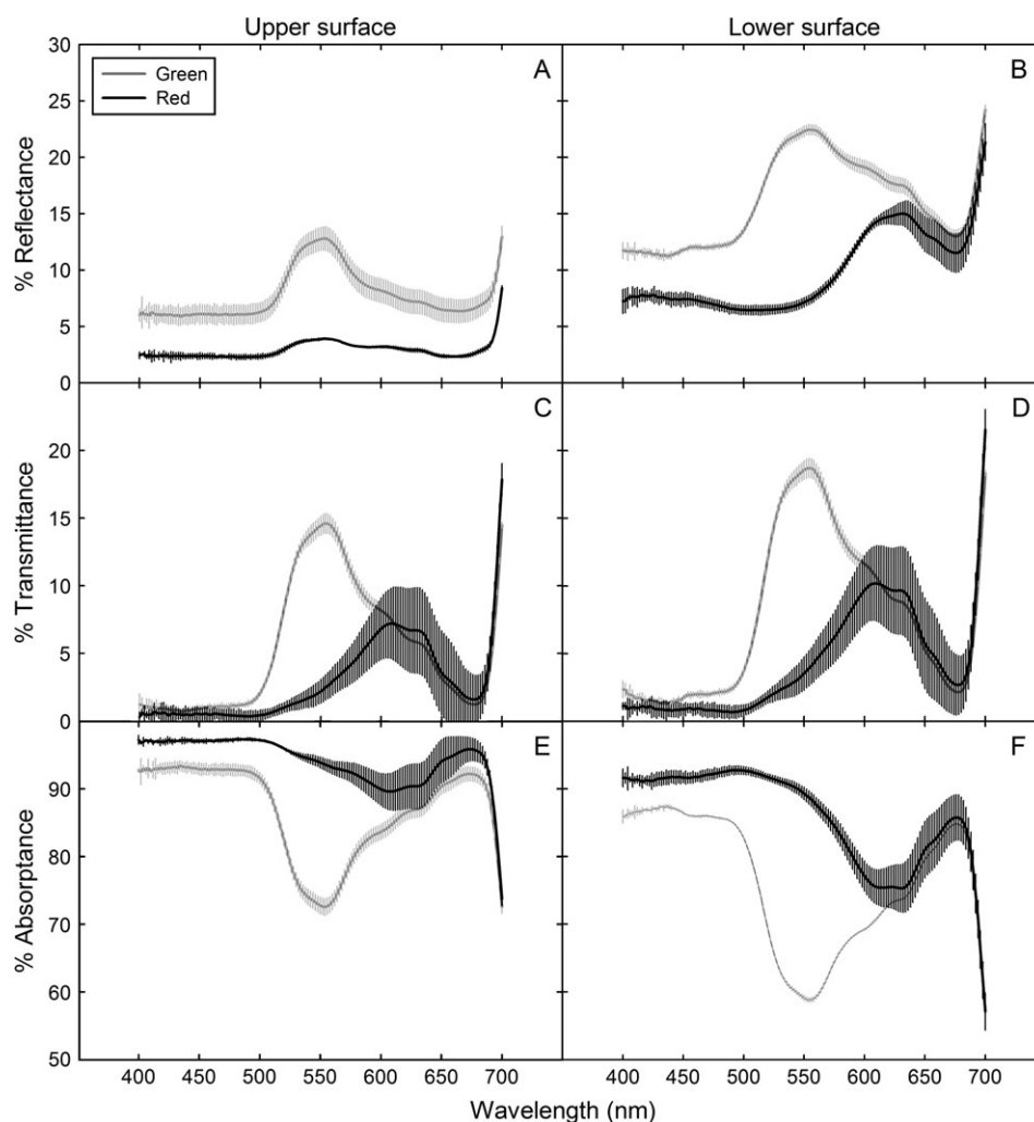
Fig. 3. Optical properties (absorbance, transmittance, and reflectance) of the adaxial and abaxial surfaces of anthocyanic (black lines) and acyanic (grey lines) tissues of Begonia heracleifolia . The lines represent the means of five leaves; error bars are 95% confidence intervals. The waveband depicted represents the visible spectrum, with violet-blue wavelengths depicted between 400–500 nm, green 500–580, yellow-orange 580–630, and red 630–700 nm.
