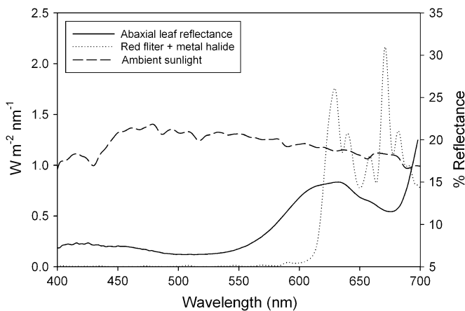
Fig. 2. Spectral scans. The solid line represents the percentage mean leaf reflectance for the red abaxial surface of Begonia heracleifolia leaves. The dotted line represents the transmission spectra for the red filter used in photosynthesis measurements. The ambient solar spectrum is represented by the dashed line.
