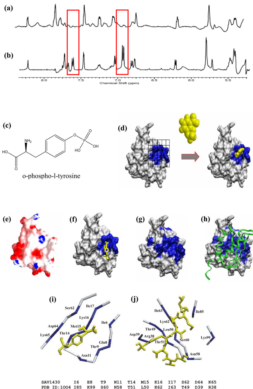
Figure 3. FAST-NMR analysis of SAV1430. Example of 1D NMR line-broadening spectra obtained in the SAV1430 screen. Expanded NMR region corresponding to the aromatic residues (a) in the presence of SAV1430 and (b) the free mixture, illustrating the binding of SAV1430 by changes in observed NMR line-widths. SAV1430 surface where residues that incur a chemical shift change are darkened. (c) Chemical structure of O -phospho-L-tyrosine shown to bind SAV1430. (d) Illustration of the use of the NMR defined ligand binding site to direct a protein-ligand co-structure determination with AutoDock 36 . (e) GRASP 37 electrostatic surface where positive and negative regions are blue and red, respectively. (f) NMR-based ligand-defined SAV1430 binding site where residues that incur a chemical shift change upon binding
