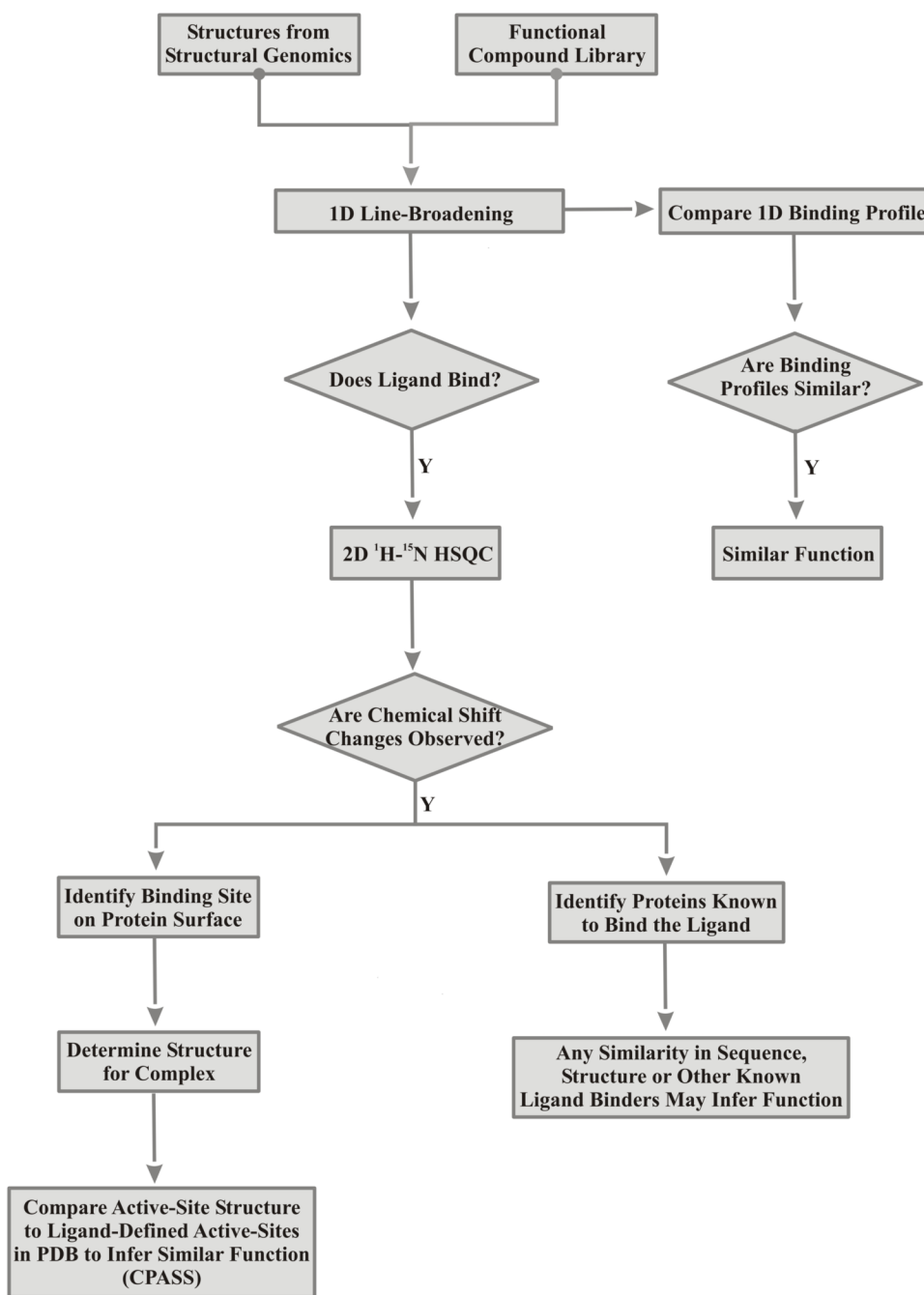
Figure 2. Flow Chart for the FAST-NMR screen.
