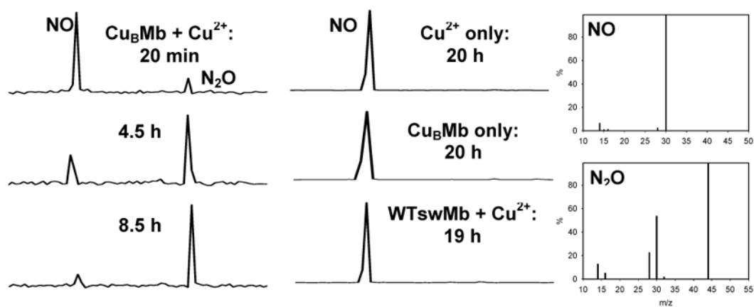
Figure 2. GC/MS chromatogram of NO reduction by Cu B Mb and Cu 2+ . The GC peaks have been normalized.
