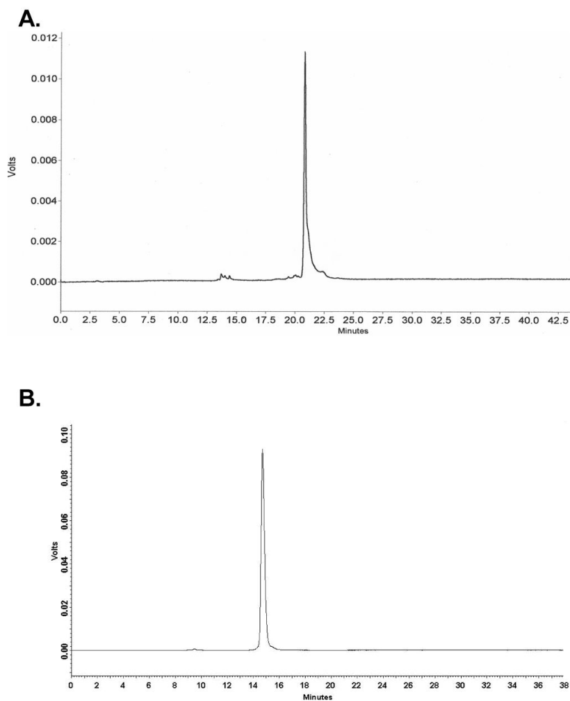
Figure 1. Reversed-phase HPLC analysis and purification of the Se-DNAs. A) the HPLC analysis profile of the crude DMTr-on Se-DNA (5'-DMTr-GT Se -GTACAC-3') after cleavage from the solid support and deprotection. The HPLC analysis was performed on a Zorbax SB-C18 column (4.6 × 250 mm) with a linear gradient from buffer A (20 mM triethylammonium acetate, pH 7.1) to 70% buffer B (50% acetonitrile, 20 mM triethyl ammonium acetate, pH 7.1) in 20 minutes; the Se-DNA retention time was 20.6 min. B) the HPLC purification profile of the DMTr-off Se-DNA (5'-GT Se -GTACAC-3'). The sample was eluted on a Zorbax SB-C18 column (21 × 250 mm; flow rate: 6 mL/min) with the same gradient and buffers; its retention time is 14.8 min.
