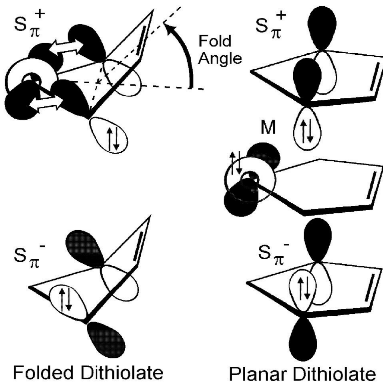
Figure 1. Representations of the valence orbitals of folded versus flat dithiolates. In the d^0 case the metal orbital (M) is empty, and the S_{\pi^+} orbital can interact upon folding. In the d^2 case the metal orbital (M) is filled, and a planar orientation minimizes a filled-filled interaction. The S_{\pi^-} orbital does not have the correct symmetry to interact with the metal orbital.
